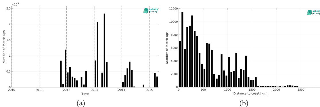
Figure 1: Number of match-ups between TSG (GOSUD-Research-vessel) and Aquarius SSS L3 OR v5 - Monthly (NASA-GSFC) SSS as a function of time (a) and as function of the distance to coast (b) over the Equatorial Ocean 10N-10S Pi-MEP region and for the full satellite product period.
