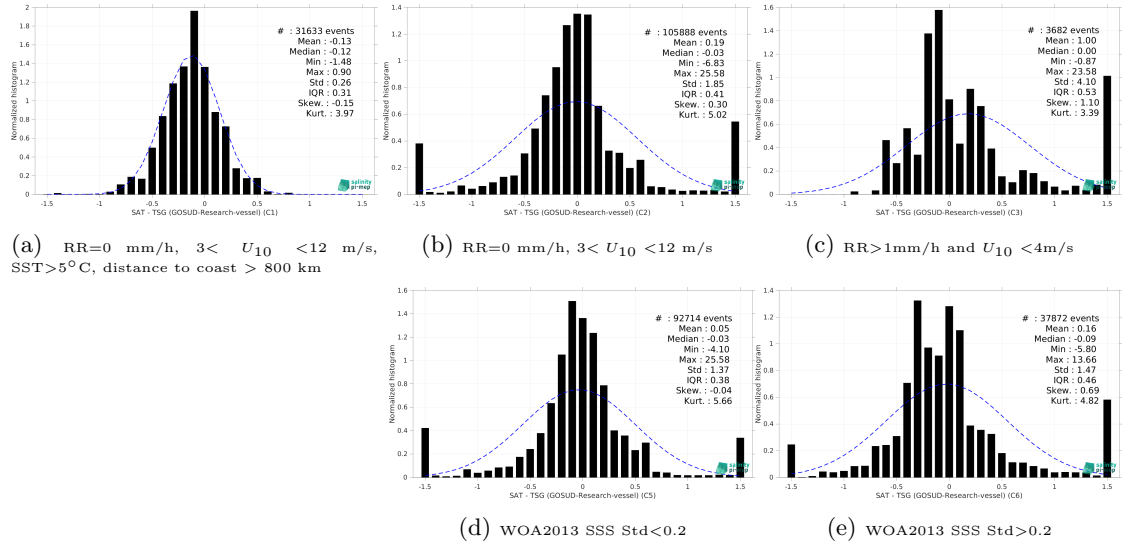
Figure 13: Normalized histogram of \Delta\text{SSS} (Aquarius SSS L3 OR v5 - Monthly (NASA-GSFC) - TSG (GOSUD-Research-vessel)) for 5 different subdatasets corresponding to: RR=0 mm/h, 3 < U_{10} < 12 m/s, SST>5°C, distance to coast > 800 km (a), RR=0 mm/h, 3 < U_{10} < 12 m/s (b), RR>1mm/h and U_{10} < 4 m/s (c), WOA2013 SSS Std<0.2 (d), WOA2013 SSS Std>0.2 (e).
