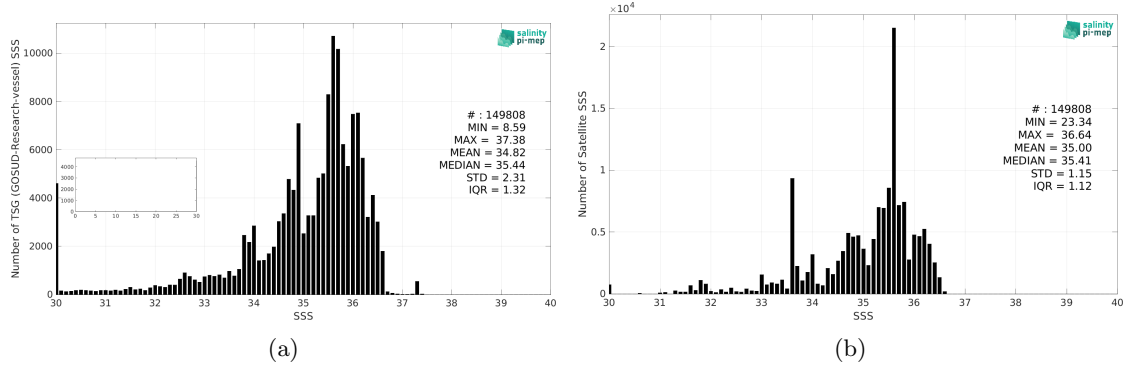
Figure 2: Histograms of SSS from TSG (GOSUD-Research-vessel) (a) and Aquarius SSS L3 OR v5 - Monthly (NASA-GSFC) (b) considering all match-up pairs per bins of 0.1 over the Equatorial Ocean 10N-10S Pi-MEP region and for the full satellite product period.
