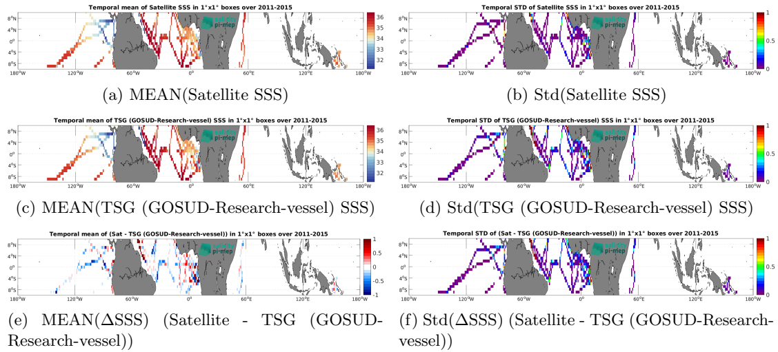
Figure 6: Temporal mean (left) and Std (right) of SSS from Aquarius SSS L3 OR v5 - Monthly (NASA-GSFC) (top), TSG (GOSUD-Research-vessel) (middle), and of \Delta SSS (Satellite - TSG (GOSUD-Research-vessel)). Only match-up pairs are used to generate these maps.
