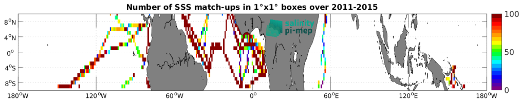
Figure 4: Number of SSS match-ups between TSG (GOSUD-Research-vessel) SSS and the Aquarius SSS L3 OR v5 - Monthly (NASA-GSFC) SSS product for the Equatorial Ocean 10N-10S Pi-MEP region over 1^\circ \times 1^\circ boxes and for the full satellite product period.
