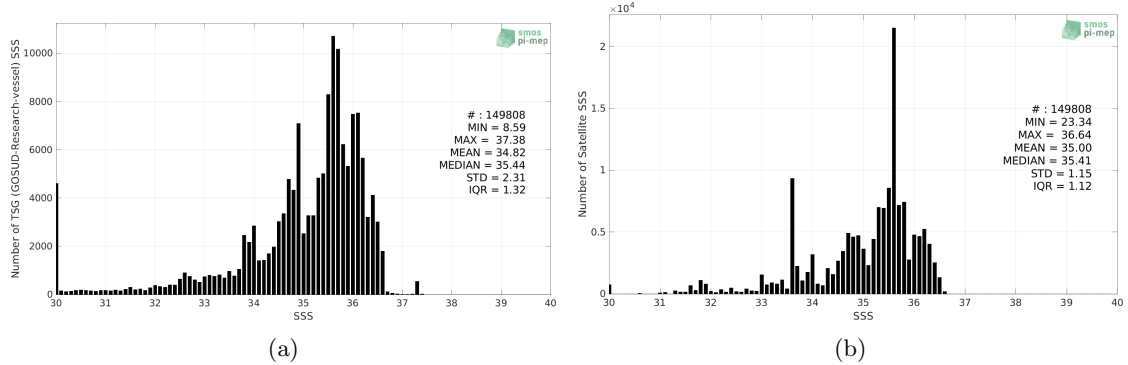
Figure 2: Histograms of SSS from TSG (GOSUD-Research-vessel) (a) and Aquarius SSS L3 OR v5 - Monthly (NASA-GSFC) (b) considering all match-up pairs per bins of 0.1 over the Equatorial Ocean 10N-10S Pi-MEP region and for the full satellite product period.
