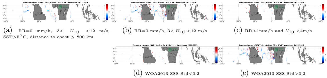
Figure 12: Temporal mean gridded over spatial boxes of size 1^{\circ}\times 1^{\circ} of \Delta SSS (Aquarius SSS L3 OR v5 - Monthly (NASA-GSFC) - TSG (GOSUD-Research-vessel)) for 5 different subdatasets corresponding to:RR=0 mm/h, 3 < U_{10} < 12 m/s, SST > 5^{\circ}\text{C} , distance to coast > 800 km (a), RR=0 mm/h, 3 < U_{10} < 12 m/s (b), RR > 1 mm/h and U_{10} < 4 m/s (c), WOA2013 SSS Std < 0.2 (d), WOA2013 SSS Std > 0.2 (e).
