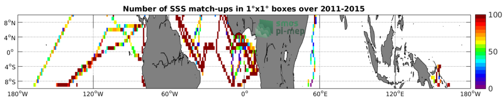
Figure 4: Number of SSS match-ups between TSG-GOSUD-Research-vessel SSS and the Aquarius-L3-OR-V5-MONTHLY-1DEG SSS product for the Equatorial Ocean 10N-10S Pi-MEP region over 1^\circ \times 1^\circ boxes and for the full satellite product period.
