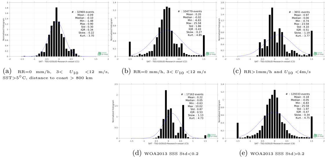
Figure 13: Normalized histogram of \Delta SSS (Aquarius-L3-OR-V5-MONTHLY-1DEG - TSG-GOSUD-Research-vessel) for 5 different subdatasets corresponding to: RR=0 mm/h, 3 < U_{10} < 12 m/s, SST >5^\circ C, distance to coast > 800 km (a), RR=0 mm/h, 3 < U_{10} < 12 m/s (b), RR >1 mm/h and U_{10} < 4 m/s (c), WOA2013 SSS Std <0.2 (d), WOA2013 SSS Std >0.2 (e).
