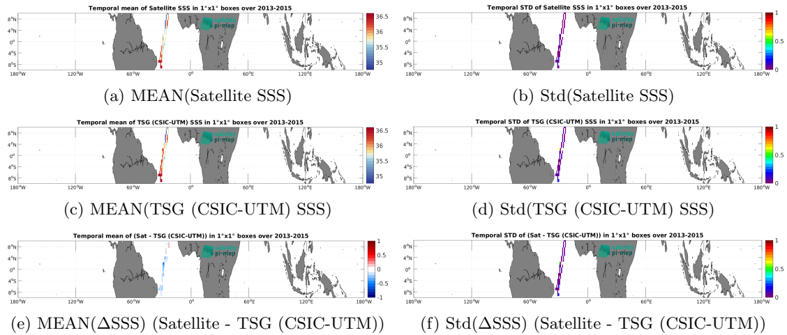
Figure 7: Temporal mean (left) and Std (right) of SSS from Aquarius SSS L3 OR v5 - Monthly (NASA-GSFC) (top), TSG (CSIC-UTM) (middle), and of \Delta SSS (Satellite - TSG (CSIC-UTM)). Only match-up pairs are used to generate these maps.
