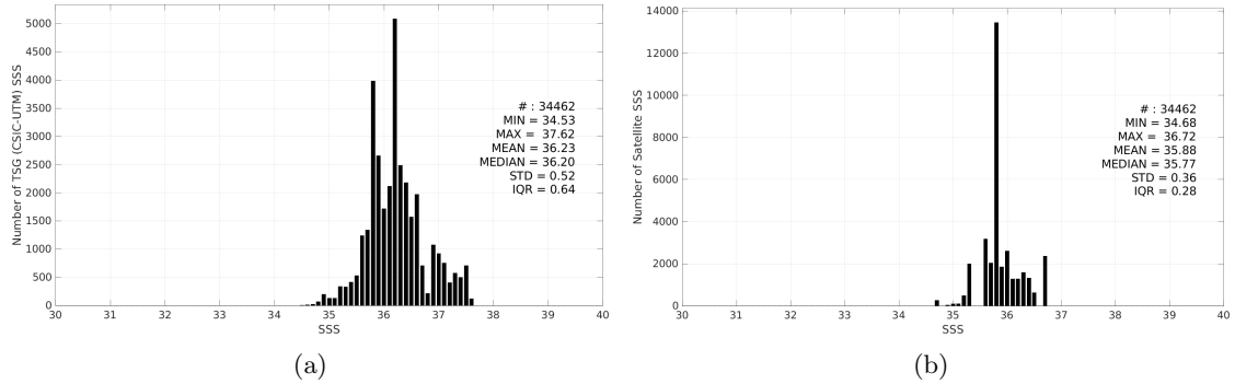
Figure 3: Histograms of SSS from TSG (CSIC-UTM) (a) and Aquarius SSS L3 OR v5 - Monthly (NASA-GSFC) (b) considering all match-up pairs per bins of 0.1 over the Equatorial Ocean 10N-10S Pi-MEP region and for the full satellite product period.
