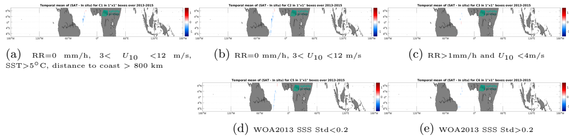
Figure 14: Temporal mean gridded over spatial boxes of size 1^\circ \times 1^\circ of \Delta SSS (Aquarius SSS L3 OR v5 - Monthly (NASA-GSFC) - TSG (CSIC-UTM)) for 5 different subdatasets corresponding to: RR=0 mm/h, 3 < U_{10} < 12 m/s, SST >5^\circ C, distance to coast > 800 km (a), RR=0 mm/h, 3 < U_{10} < 12 m/s (b), RR >1 mm/h and U_{10} < 4 m/s (c), WOA2013 SSS Std <0.2 (d), WOA2013 SSS Std >0.2 (e).
