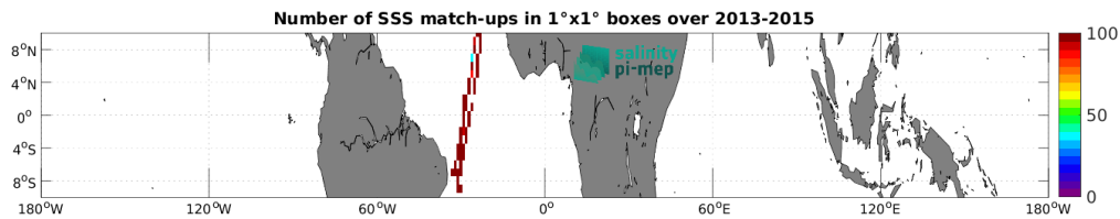
Figure 5: Number of SSS match-ups between TSG (CSIC-UTM) SSS and the Aquarius SSS L3 OR v5 - Monthly (NASA-GSFC) SSS product for the Equatorial Ocean 10N-10S Pi-MEP region over 1^\circ \times 1^\circ boxes and for the full satellite product period.
