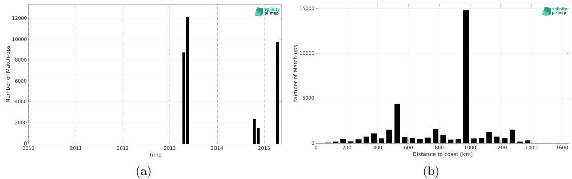
Figure 2: Number of match-ups between TSG (CSIC-UTM) and Aquarius SSS L3 OR v5 - Monthly (NASA-GSFC) SSS as a function of time (a) and as function of the distance to coast (b) over the Equatorial Ocean 10N-10S Pi-MEP region and for the full satellite product period.
