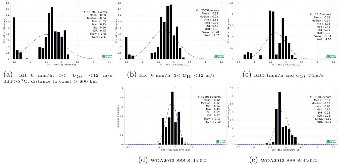
Figure 15: Normalized histogram of \Delta SSS (Aquarius SSS L3 OR v5 - Monthly (NASA-GSFC) - TSG (CSIC-UTM)) for 5 different subdatasets corresponding to: RR=0 mm/h, 3 < U_{10} < 12 m/s, SST >5^\circ C, distance to coast > 800 km (a), RR=0 mm/h, 3 < U_{10} < 12 m/s (b), RR >1 mm/h and U_{10} < 4 m/s (c), WOA2013 SSS Std <0.2 (d), WOA2013 SSS Std >0.2 (e).
