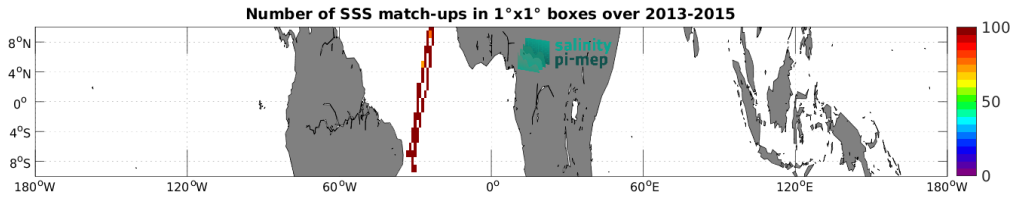
Figure 4: Number of SSS match-ups between TSG (CSIC-UTM) SSS and the Aquarius SSS L3 OR v5 - Monthly (NASA-GSFC) SSS product for the Equatorial Ocean 10N-10S Pi-MEP region over 1^\circ \times 1^\circ boxes and for the full satellite product period.
