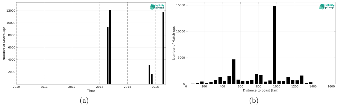
Figure 1: Number of match-ups between TSG (CSIC-UTM) and Aquarius SSS L3 OR v5 - Monthly (NASA-GSFC) SSS as a function of time (a) and as function of the distance to coast (b) over the Equatorial Ocean 10N-10S Pi-MEP region and for the full satellite product period.
