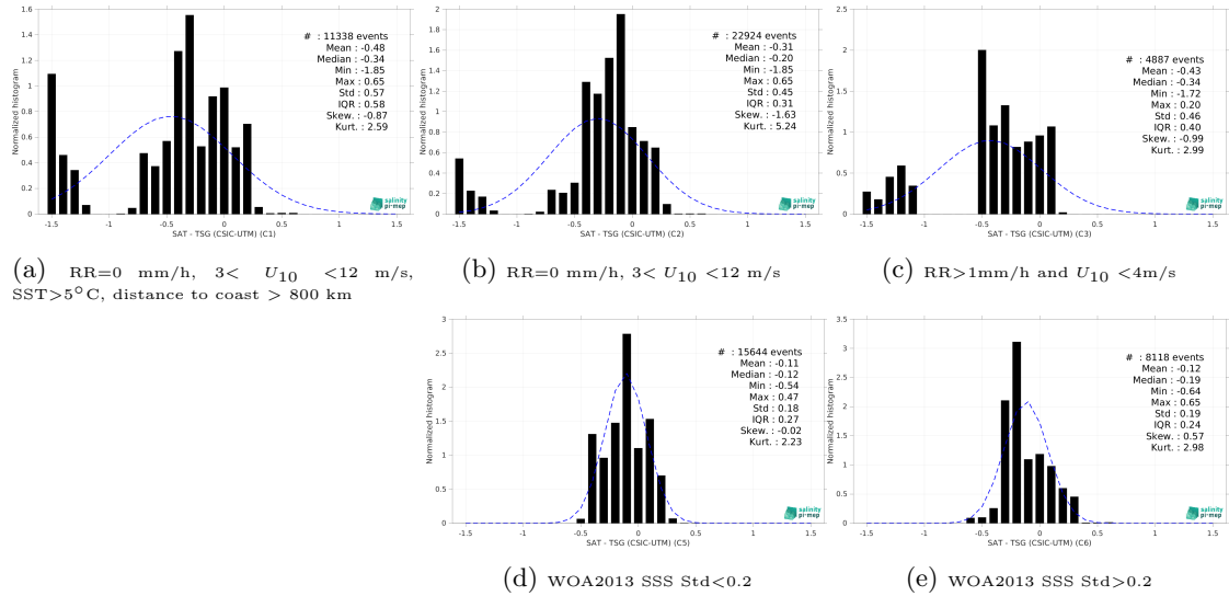
Figure 13: Normalized histogram of \Delta SSS (Aquarius SSS L3 OR v5 - Monthly (NASA-GSFC) - TSG (CSIC-UTM)) for 5 different subdatasets corresponding to: RR=0 mm/h, 3 < U_{10} < 12 m/s, SST >5^\circ C, distance to coast > 800 km (a), RR=0 mm/h, 3 < U_{10} < 12 m/s (b), RR >1 mm/h and U_{10} < 4 m/s (c), WOA2013 SSS Std <0.2 (d), WOA2013 SSS Std >0.2 (e).
