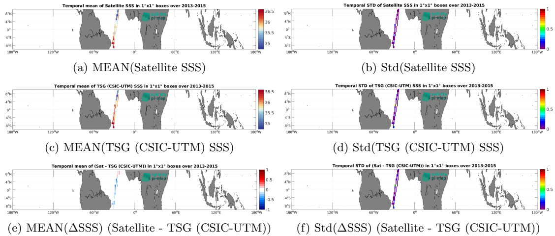
Figure 6: Temporal mean (left) and Std (right) of SSS from Aquarius SSS L3 OR v5 - Monthly (NASA-GSFC) (top), TSG (CSIC-UTM) (middle), and of \Delta SSS (Satellite - TSG (CSIC-UTM)). Only match-up pairs are used to generate these maps.
