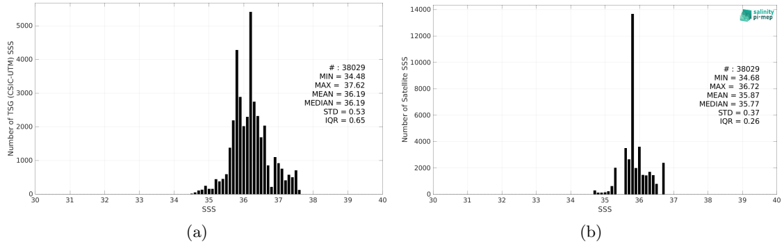
Figure 2: Histograms of SSS from TSG (CSIC-UTM) (a) and Aquarius SSS L3 OR v5 - Monthly (NASA-GSFC) (b) considering all match-up pairs per bins of 0.1 over the Equatorial Ocean 10N-10S Pi-MEP region and for the full satellite product period.
