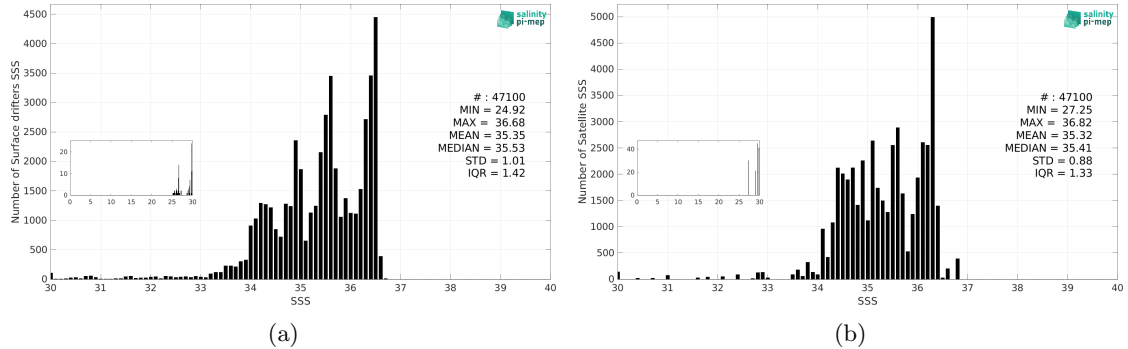
Figure 3: Histograms of SSS from Surface drifters (a) and Aquarius SSS L3 OR v5 - Monthly (NASA-GSFC) (b) considering all match-up pairs per bins of 0.1 over the Equatorial Ocean 10N-10S Pi-MEP region and for the full satellite product period.
