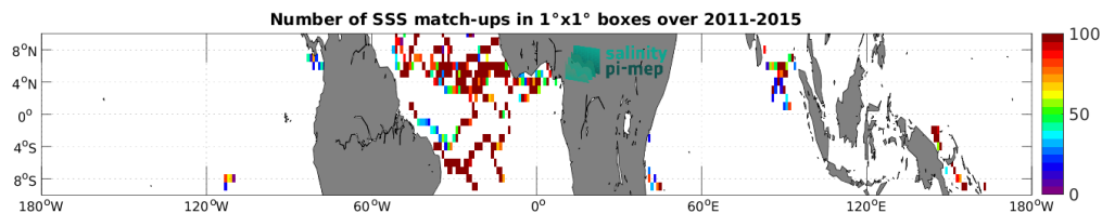
Figure 4: Number of SSS match-ups between Surface drifters SSS and the Aquarius SSS L3 OR v5 - Monthly (NASA-GSFC) SSS product for the Equatorial Ocean 10N-10S Pi-MEP region over 1^\circ \times 1^\circ boxes and for the full satellite product period.
