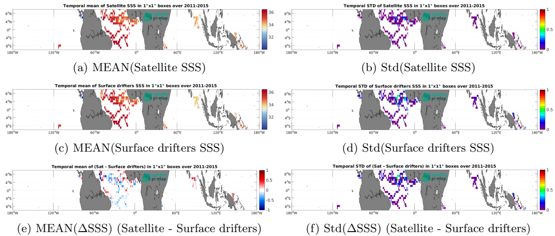
Figure 6: Temporal mean (left) and Std (right) of SSS from Aquarius SSS L3 OR v5 - Monthly (NASA-GSFC) (top), Surface drifters (middle), and of \Delta SSS (Satellite - Surface drifters). Only match-up pairs are used to generate these maps.
