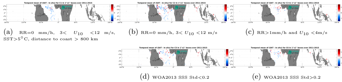
Figure 13: Temporal mean gridded over spatial boxes of size 1^\circ \times 1^\circ of \Delta SSS (Aquarius SSS L3 OR v5 - Monthly (NASA-GSFC) - Surface drifters) for 5 different subdatasets corresponding to: RR=0 mm/h, 3 < U_{10} < 12 m/s, SST >5^\circ\text{C} , distance to coast > 800 km (a), RR=0 mm/h, 3 < U_{10} < 12 m/s (b), RR >1 mm/h and U_{10} < 4 m/s (c), WOA2013 SSS Std <0.2 (d), WOA2013 SSS Std >0.2 (e).
