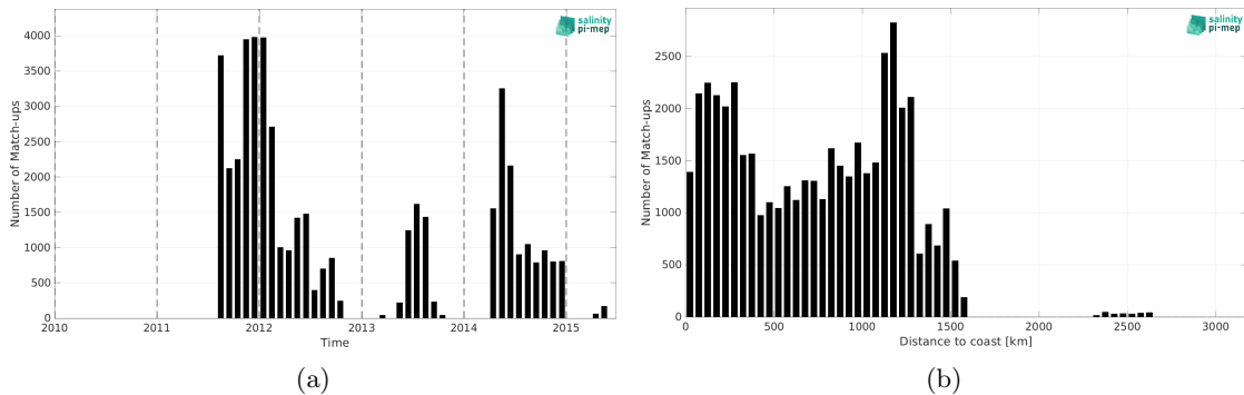
Figure 2: Number of match-ups between Surface drifters and Aquarius SSS L3 OR v5 - Monthly (NASA-GSFC) SSS as a function of time (a) and as function of the distance to coast (b) over the Equatorial Ocean 10N-10S Pi-MEP region and for the full satellite product period.
