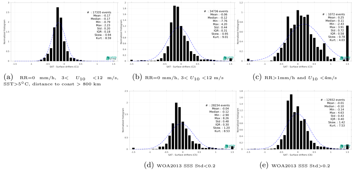
Figure 14: Normalized histogram of \Delta SSS (Aquarius SSS L3 OR v5 - Monthly (NASA-GSFC) - Surface drifters) for 5 different subdatasets corresponding to: RR=0 mm/h, 3 < U_{10} < 12 m/s, SST >5^\circ\text{C} , distance to coast > 800 km (a), RR=0 mm/h, 3 < U_{10} < 12 m/s (b), RR >1 mm/h and U_{10} < 4 m/s (c), WOA2013 SSS Std <0.2 (d), WOA2013 SSS Std >0.2 (e).
