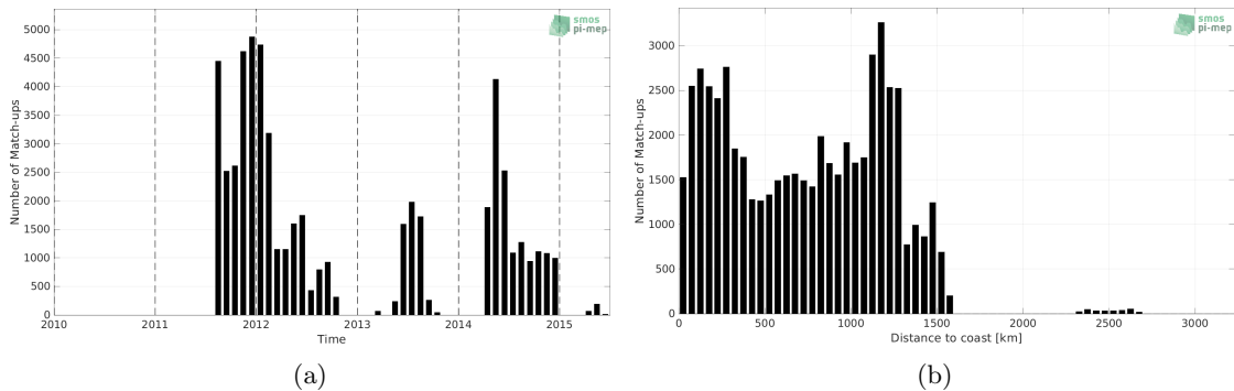
Figure 1: Number of match-ups between Surface drifters and Aquarius SSS L3 OR v5 - Monthly (NASA-GSFC) SSS as a function of time (a) and as function of the distance to coast (b) over the Equatorial Ocean 10N-10S Pi-MEP region and for the full satellite product period.
