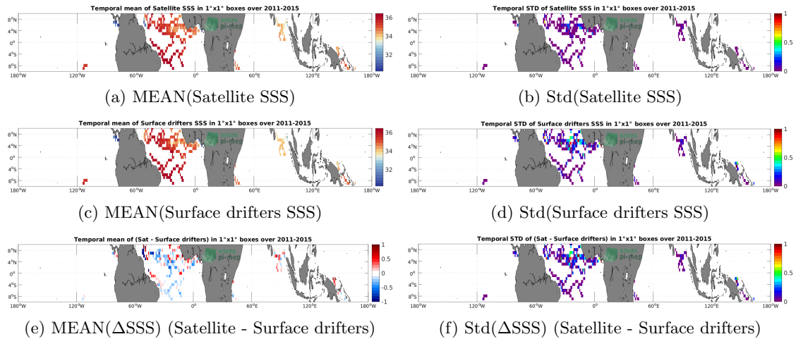
Figure 5: Temporal mean (left) and Std (right) of SSS from Aquarius SSS L3 OR v5 - Monthly (NASA-GSFC) (top), Surface drifters (middle), and of \Delta SSS (Satellite - Surface drifters). Only match-up pairs are used to generate these maps.
