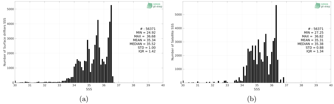
Figure 2: Histograms of SSS from Surface drifters (a) and Aquarius SSS L3 OR v5 - Monthly (NASA-GSFC) (b) considering all match-up pairs per bins of 0.1 over the Equatorial Ocean 10N-10S Pi-MEP region and for the full satellite product period.
