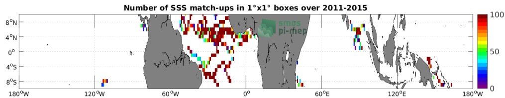
Figure 3: Number of SSS match-ups between Surface drifters SSS and the Aquarius SSS L3 OR v5 - Monthly (NASA-GSFC) SSS product for the Equatorial Ocean 10N-10S Pi-MEP region over 1^\circ \times 1^\circ boxes and for the full satellite product period.
