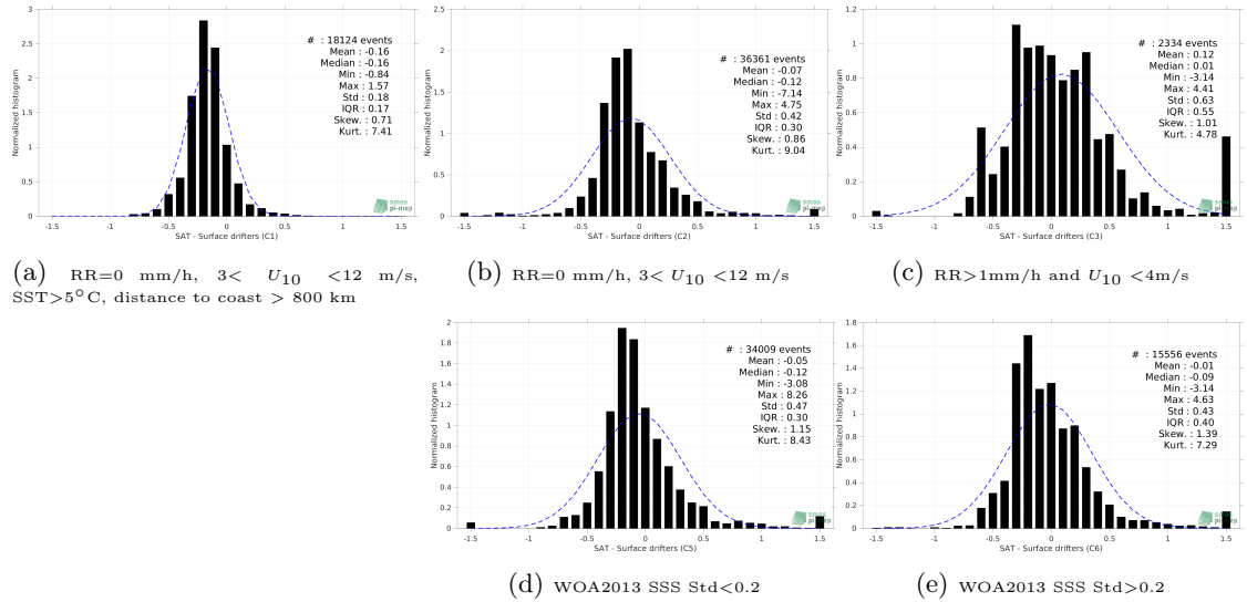
Figure 12: Normalized histogram of \Delta SSS (Aquarius SSS L3 OR v5 - Monthly (NASA-GSFC) - Surface drifters) for 5 different subdatasets corresponding to: RR=0 mm/h, 3 < U_{10} < 12 m/s, SST >5^\circ\text{C} , distance to coast > 800 km (a), RR=0 mm/h, 3 < U_{10} < 12 m/s (b), RR >1 mm/h and U_{10} < 4 m/s (c), WOA2013 SSS Std <0.2 (d), WOA2013 SSS Std >0.2 (e).
