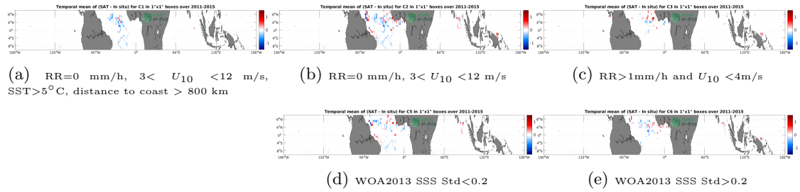
Figure 11: Temporal mean gridded over spatial boxes of size 1^\circ \times 1^\circ of \Delta SSS (Aquarius SSS L3 OR v5 - Monthly (NASA-GSFC) - Surface drifters) for 5 different subdatasets corresponding to: RR=0 mm/h, 3 < U_{10} < 12 m/s, SST >5^\circ\text{C} , distance to coast > 800 km (a), RR=0 mm/h, 3 < U_{10} < 12 m/s (b), RR >1 mm/h and U_{10} < 4 m/s (c), WOA2013 SSS Std <0.2 (d), WOA2013 SSS Std >0.2 (e).
