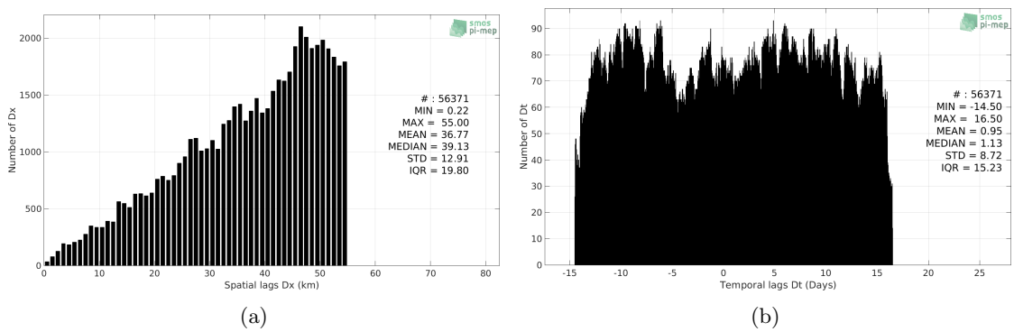
Figure 4: Histograms of the spatial (a) and temporal (b) lags between the time of the Surface drifters measurements and the date of the corresponding Aquarius-L3-OR-V5-MONTHLY-1DEG SSS product.
