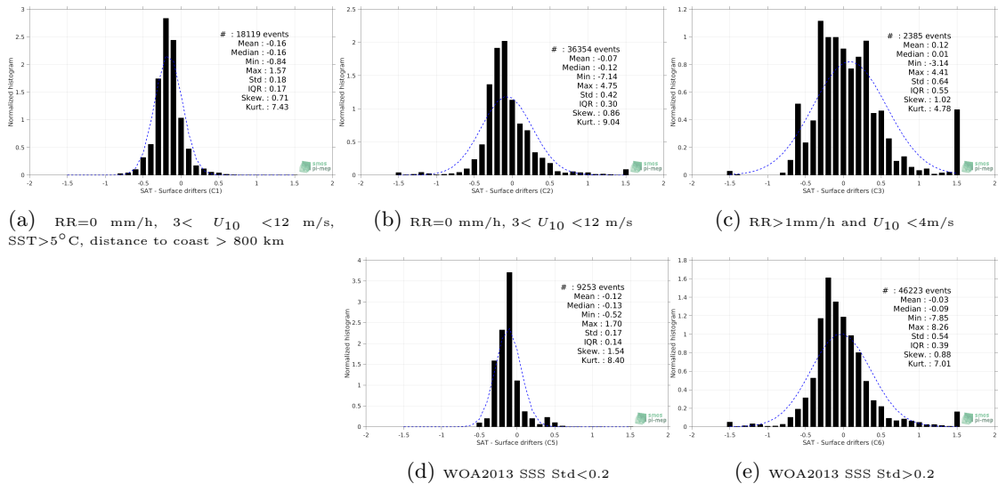
Figure 12: Normalized histogram of \Delta SSS (Aquarius-L3-OR-V5-MONTHLY-1DEG - Surface drifters) for 5 different subdatasets corresponding to: RR=0 mm/h, 3 < U_{10} < 12 m/s, SST >5^\circ C, distance to coast > 800 km (a), RR=0 mm/h, 3 < U_{10} < 12 m/s (b), RR >1 mm/h and U_{10} < 4 m/s (c), WOA2013 SSS Std <0.2 (d), WOA2013 SSS Std >0.2 (e).
