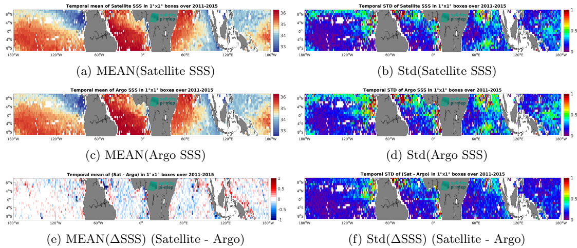
Figure 7: Temporal mean (left) and Std (right) of SSS from Aquarius SSS L3 OR v5 - Monthly (NASA-GSFC) (top), Argo (middle), and of \Delta SSS (Satellite - Argo). Only match-up pairs are used to generate these maps.
