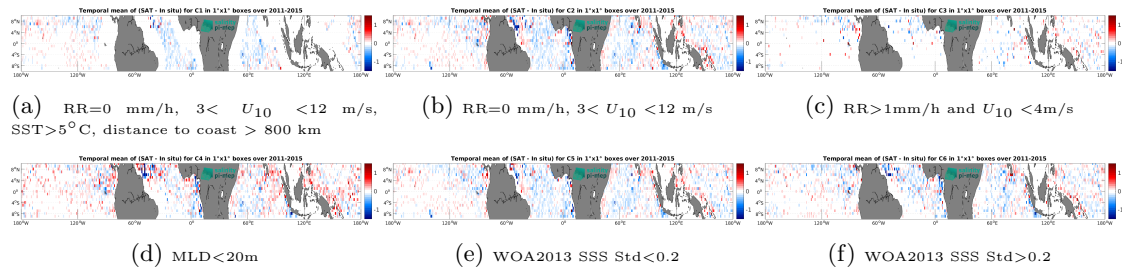
Figure 14: Temporal mean gridded over spatial boxes of size 1^\circ \times 1^\circ of \Delta SSS (Aquarius SSS L3 OR v5 - Monthly (NASA-GSFC) - Argo) for 6 different subdatasets corresponding to:RR=0 mm/h, 3 < U_{10} < 12 m/s, SST >5^\circ C, distance to coast > 800 km (a), RR=0 mm/h, 3 < U_{10} < 12 m/s (b), RR >1 mm/h and U_{10} < 4 m/s (c),MLD <20 m (d),WOA2013 SSS Std <0.2 (e),WOA2013 SSS Std >0.2 (f).
