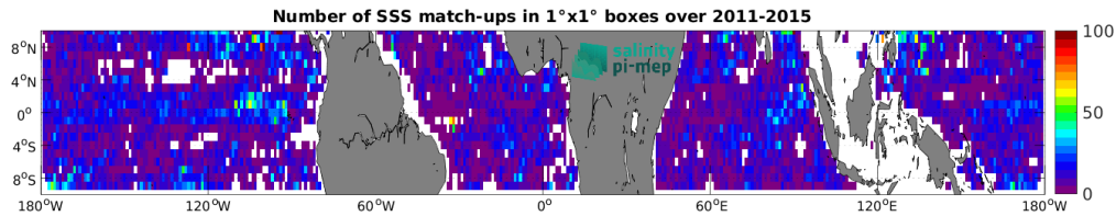
Figure 5: Number of SSS match-ups between Argo SSS and the Aquarius SSS L3 OR v5 - Monthly (NASA-GSFC) SSS product for the Equatorial Ocean 10N-10S Pi-MEP region over 1^\circ \times 1^\circ boxes and for the full satellite product period.
