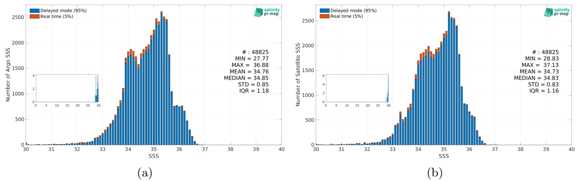
Figure 3: Histograms of SSS from Argo (a) and Aquarius SSS L3 OR v5 - Monthly (NASA-GSFC) (b) considering all match-up pairs per bins of 0.1 over the Equatorial Ocean 10N-10S Pi-MEP region and for the full satellite product period.
