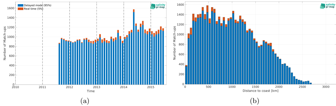
Figure 2: Number of match-ups between Argo and Aquarius SSS L3 OR v5 - Monthly (NASA-GSFC) SSS as a function of time (a) and as function of the distance to coast (b) over the Equatorial Ocean 10N-10S Pi-MEP region and for the full satellite product period.
