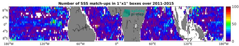
Figure 4: Number of SSS match-ups between Argo SSS and the Aquarius SSS L3 OR v5 - Monthly (NASA-GSFC) SSS product for the Equatorial Ocean 10N-10S Pi-MEP region over 1^\circ \times 1^\circ boxes and for the full satellite product period.
