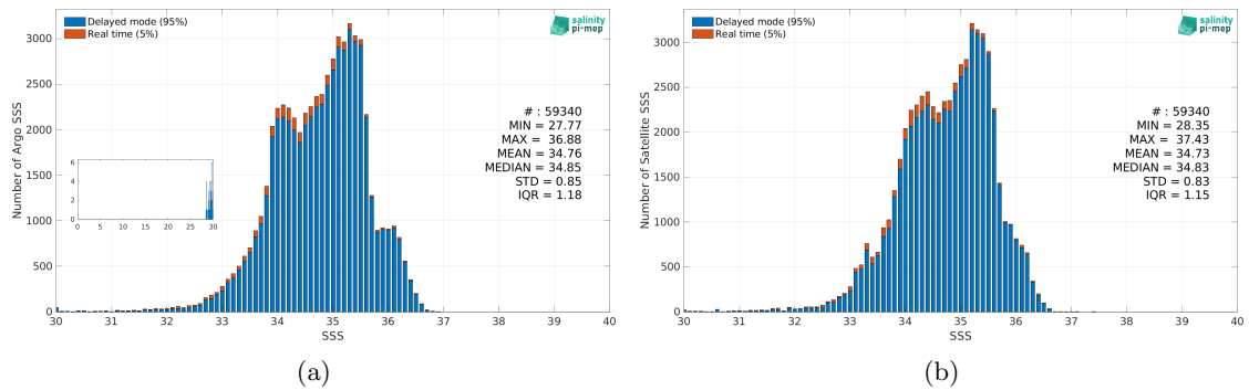
Figure 2: Histograms of SSS from Argo (a) and Aquarius SSS L3 OR v5 - Monthly (NASA-GSFC) (b) considering all match-up pairs per bins of 0.1 over the Equatorial Ocean 10N-10S Pi-MEP region and for the full satellite product period.
