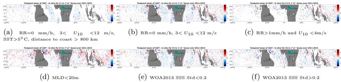
Figure 12: Temporal mean gridded over spatial boxes of size 1^\circ \times 1^\circ of \Delta SSS (Aquarius SSS L3 OR v5 - Monthly (NASA-GSFC) - Argo) for 6 different subdatasets corresponding to:RR=0 mm/h, 3 < U_{10} < 12 m/s, SST >5^\circ C, distance to coast > 800 km (a), RR=0 mm/h, 3 < U_{10} < 12 m/s (b), RR >1 mm/h and U_{10} < 4 m/s (c),MLD <20 m (d),WOA2013 SSS Std <0.2 (e),WOA2013 SSS Std >0.2 (f).
