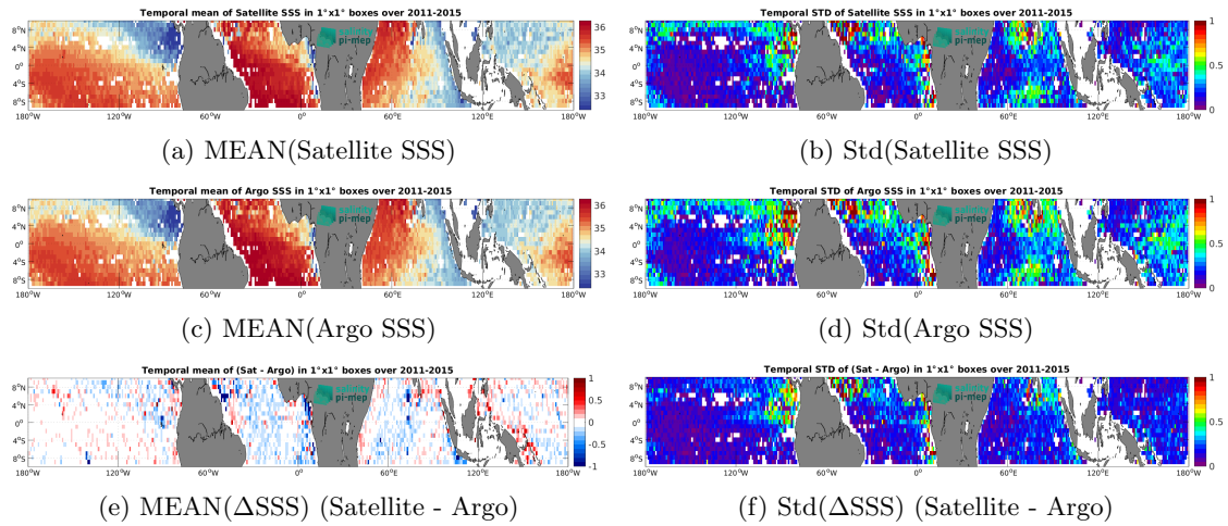
Figure 6: Temporal mean (left) and Std (right) of SSS from Aquarius SSS L3 OR v5 - Monthly (NASA-GSFC) (top), Argo (middle), and of \Delta SSS (Satellite - Argo). Only match-up pairs are used to generate these maps.
