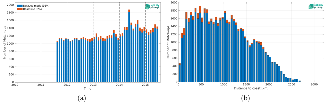
Figure 1: Number of match-ups between Argo and Aquarius SSS L3 OR v5 - Monthly (NASA-GSFC) SSS as a function of time (a) and as function of the distance to coast (b) over the Equatorial Ocean 10N-10S Pi-MEP region and for the full satellite product period.
