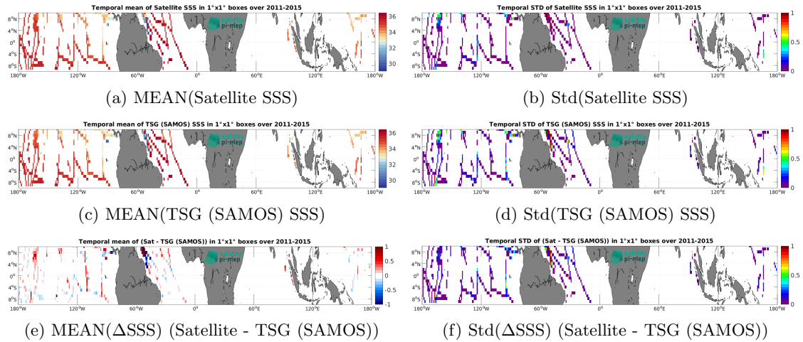
Figure 7: Temporal mean (left) and Std (right) of SSS from Aquarius SSS L3 OR v5 - Monthly - Rain mask (NASA-GSFC) (top), TSG (SAMOS) (middle), and of \Delta SSS (Satellite - TSG (SAMOS)). Only match-up pairs are used to generate these maps.
