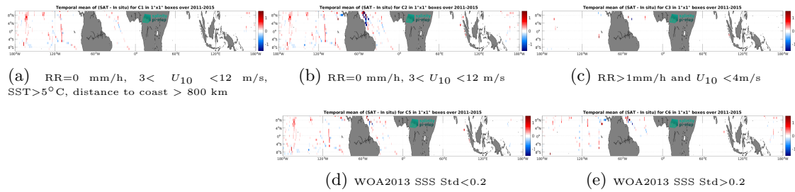
Figure 14: Temporal mean gridded over spatial boxes of size 1^\circ \times 1^\circ of \Delta SSS (Aquarius SSS L3 OR v5 - Monthly - Rain mask (NASA-GSFC) - TSG (SAMOS)) for 5 different subdatasets corresponding to:RR=0 mm/h, 3 < U_{10} < 12 m/s, SST>5°C, distance to coast > 800 km (a), RR=0 mm/h, 3 < U_{10} < 12 m/s (b), RR>1mm/h and U_{10} < 4 m/s (c), WOA2013 SSS Std<0.2 (d), WOA2013 SSS Std>0.2 (e).
