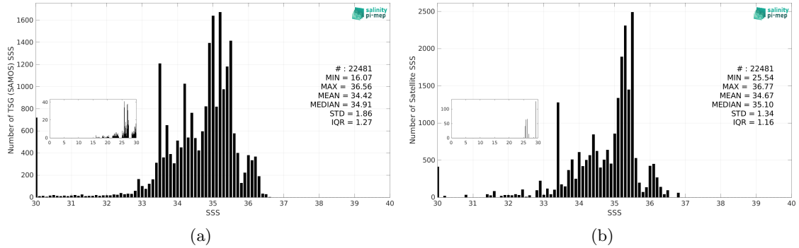
Figure 3: Histograms of SSS from TSG (SAMOS) (a) and Aquarius SSS L3 OR v5 - Monthly - Rain mask (NASA-GSFC) (b) considering all match-up pairs per bins of 0.1 over the Equatorial Ocean 10N-10S Pi-MEP region and for the full satellite product period.
