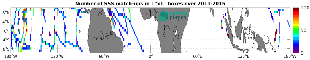
Figure 5: Number of SSS match-ups between TSG (SAMOS) SSS and the Aquarius SSS L3 OR v5 - Monthly - Rain mask (NASA-GSFC) SSS product for the Equatorial Ocean 10N-10S Pi-MEP region over 1^\circ \times 1^\circ boxes and for the full satellite product period.
