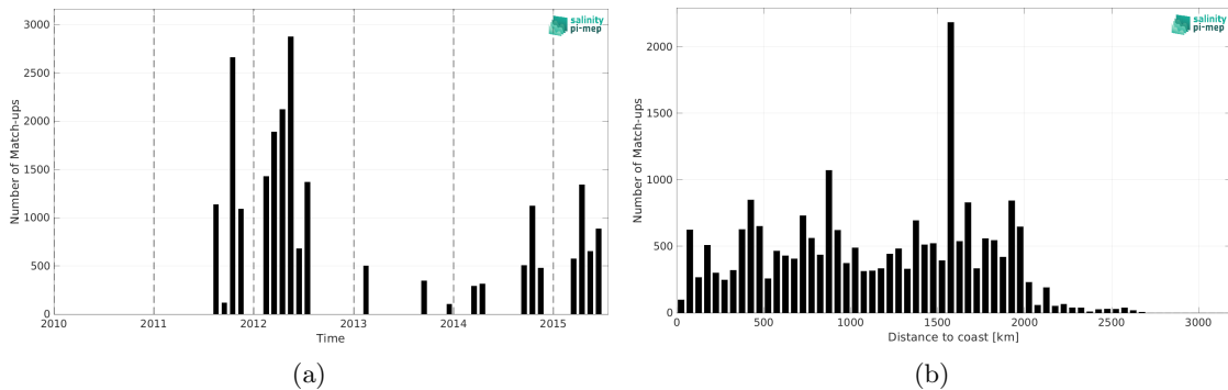
Figure 2: Number of match-ups between TSG (SAMOS) and Aquarius SSS L3 OR v5 - Monthly - Rain mask (NASA-GSFC) SSS as a function of time (a) and as function of the distance to coast (b) over the Equatorial Ocean 10N-10S Pi-MEP region and for the full satellite product period.
