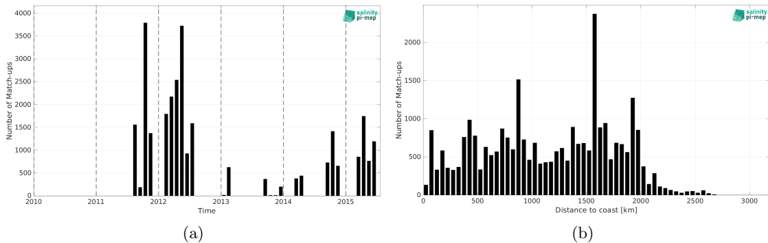
Figure 1: Number of match-ups between TSG (SAMOS) and Aquarius SSS L3 OR v5 - Monthly - Rain mask (NASA-GSFC) SSS as a function of time (a) and as function of the distance to coast (b) over the Equatorial Ocean 10N-10S Pi-MEP region and for the full satellite product period.
