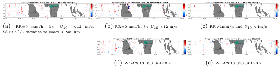
Figure 12: Temporal mean gridded over spatial boxes of size 1^\circ \times 1^\circ of \Delta SSS (Aquarius SSS L3 OR v5 - Monthly - Rain mask (NASA-GSFC) - TSG (SAMOS)) for 5 different subdatasets corresponding to: RR=0 mm/h, 3 < U_{10} < 12 m/s, SST >5^\circ\text{C} , distance to coast > 800 km (a), RR=0 mm/h, 3 < U_{10} < 12 m/s (b), RR >1 mm/h and U_{10} < 4 m/s (c), WOA2013 SSS Std <0.2 (d), WOA2013 SSS Std >0.2 (e).
