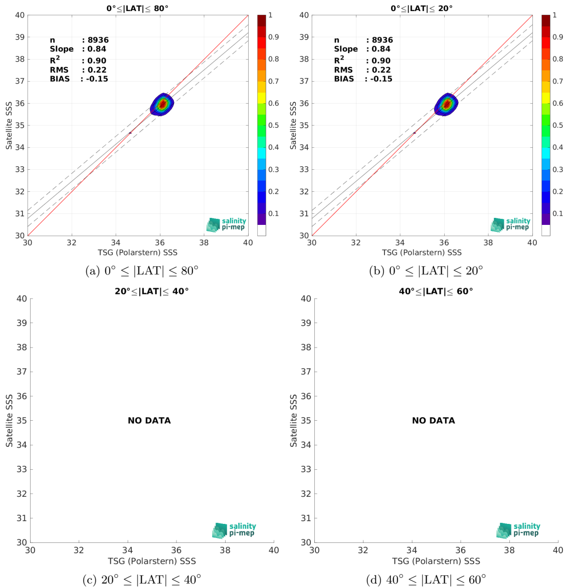
Figure 10: Contour maps of the concentration of Aquarius SSS L3 OR v5 - Monthly - Rain mask (NASA-GSFC) SSS (y-axis) versus TSG (Polarstern) SSS (x-axis) at match-up pairs for different latitude bands. For each plot, the red line shows x=y . The black thin and dashed lines indicate a linear fit through the data cloud and the \pm 95\% confidence levels, respectively. The number match-up pairs n , the slope and R^2 coefficient of the linear fit, the root mean square (RMS) and the mean bias between satellite and in situ data are indicated for each latitude band in each plots.
