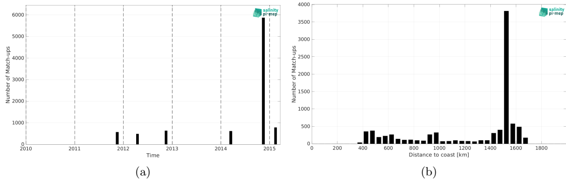
Figure 2: Number of match-ups between TSG (Polarstern) and Aquarius SSS L3 OR v5 - Monthly - Rain mask (NASA-GSFC) SSS as a function of time (a) and as function of the distance to coast (b) over the Equatorial Ocean 10N-10S Pi-MEP region and for the full satellite product period.
