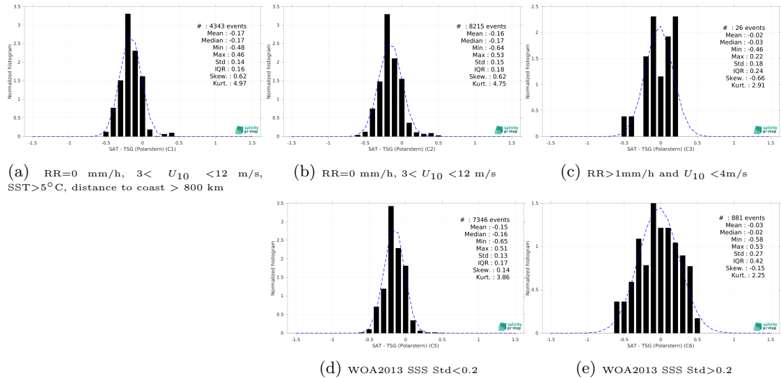
Figure 15: Normalized histogram of \Delta\text{SSS} (Aquarius SSS L3 OR v5 - Monthly - Rain mask (NASA-GSFC) - TSG (Polarstern)) for 5 different subdatasets corresponding to: RR=0 mm/h, 3 < U_{10} < 12 m/s, SST>5°C, distance to coast > 800 km (a), RR=0 mm/h, 3 < U_{10} < 12 m/s (b), RR>1mm/h and U_{10} < 4 m/s (c), WOA2013 SSS Std<0.2 (d), WOA2013 SSS Std>0.2 (e).
