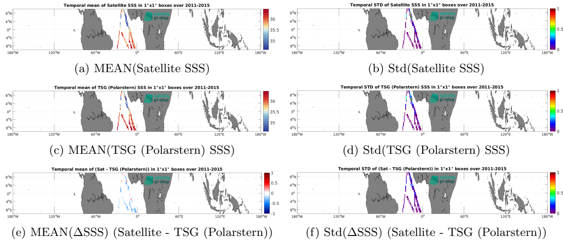
Figure 7: Temporal mean (left) and Std (right) of SSS from Aquarius SSS L3 OR v5 - Monthly - Rain mask (NASA-GSFC) (top), TSG (Polarstern) (middle), and of \Delta SSS (Satellite - TSG (Polarstern)). Only match-up pairs are used to generate these maps.
