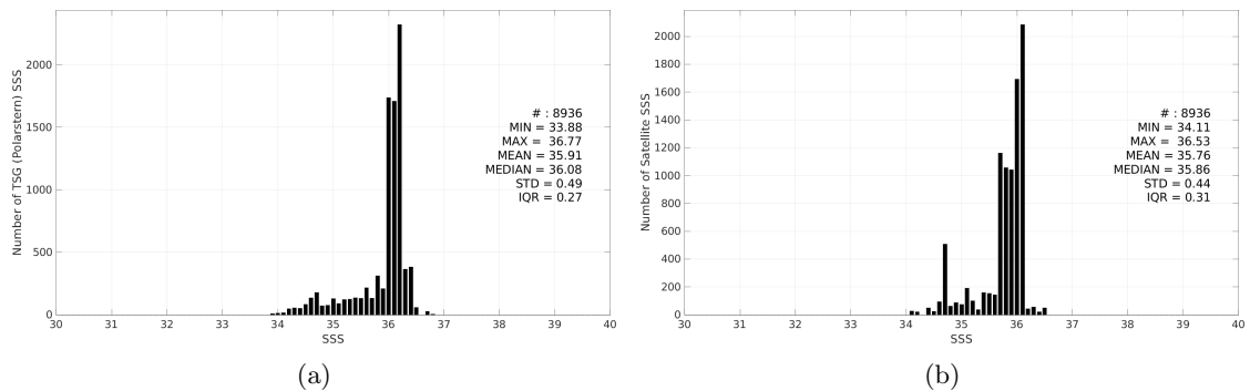
Figure 3: Histograms of SSS from TSG (Polarstern) (a) and Aquarius SSS L3 OR v5 - Monthly - Rain mask (NASA-GSFC) (b) considering all match-up pairs per bins of 0.1 over the Equatorial Ocean 10N-10S Pi-MEP region and for the full satellite product period.
