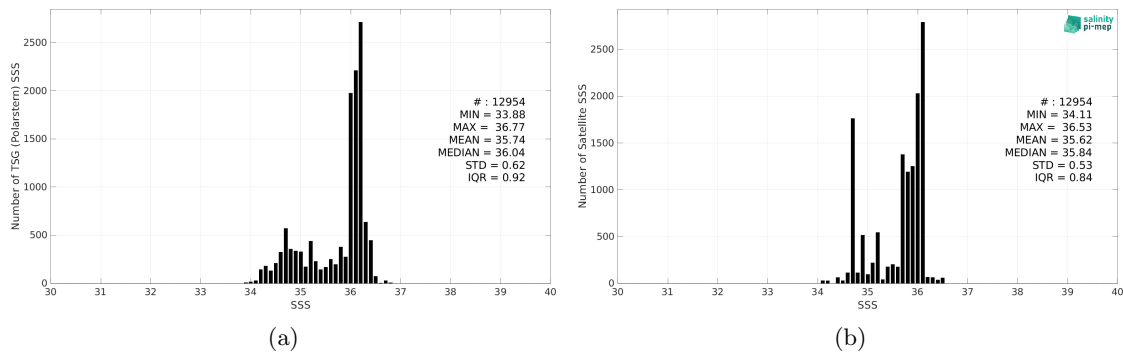
Figure 2: Histograms of SSS from TSG (Polarstern) (a) and Aquarius SSS L3 OR v5 - Monthly - Rain mask (NASA-GSFC) (b) considering all match-up pairs per bins of 0.1 over the Equatorial Ocean 10N-10S Pi-MEP region and for the full satellite product period.
