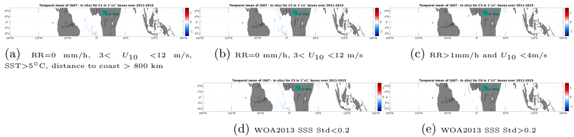
Figure 12: Temporal mean gridded over spatial boxes of size 1^{\circ}\times 1^{\circ} of \Delta\text{SSS} (Aquarius SSS L3 OR v5 - Monthly - Rain mask (NASA-GSFC) - TSG (Polarstern)) for 5 different subdatasets corresponding to:RR=0 mm/h, 3 < U_{10} < 12 m/s, SST >5^{\circ}\text{C} , distance to coast > 800 km (a), RR=0 mm/h, 3 < U_{10} < 12 m/s (b), RR >1 mm/h and U_{10} < 4 m/s (c), WOA2013 SSS Std <0.2 (d), WOA2013 SSS Std >0.2 (e).
