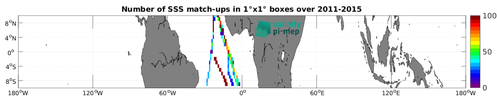
Figure 4: Number of SSS match-ups between TSG (Polarstern) SSS and the Aquarius SSS L3 OR v5 - Monthly - Rain mask (NASA-GSFC) SSS product for the Equatorial Ocean 10N-10S Pi-MEP region over 1^\circ \times 1^\circ boxes and for the full satellite product period.
