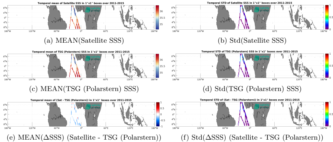
Figure 6: Temporal mean (left) and Std (right) of SSS from Aquarius SSS L3 OR v5 - Monthly - Rain mask (NASA-GSFC) (top), TSG (Polarstern) (middle), and of \Delta SSS (Satellite - TSG (Polarstern)). Only match-up pairs are used to generate these maps.
