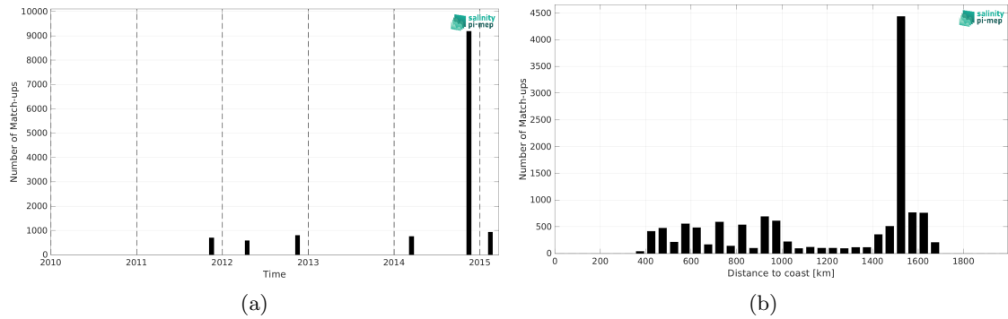
Figure 1: Number of match-ups between TSG (Polarstern) and Aquarius SSS L3 OR v5 - Monthly - Rain mask (NASA-GSFC) SSS as a function of time (a) and as function of the distance to coast (b) over the Equatorial Ocean 10N-10S Pi-MEP region and for the full satellite product period.
