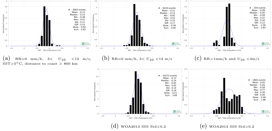
Figure 13: Normalized histogram of \Delta\text{SSS} (Aquarius SSS L3 OR v5 - Monthly - Rain mask (NASA-GSFC) - TSG (Polarstern)) for 5 different subdatasets corresponding to: RR=0 mm/h, 3 < U_{10} < 12 m/s, SST>5°C, distance to coast > 800 km (a), RR=0 mm/h, 3 < U_{10} < 12 m/s (b), RR>1mm/h and U_{10} < 4 m/s (c), WOA2013 SSS Std<0.2 (d), WOA2013 SSS Std>0.2 (e).
