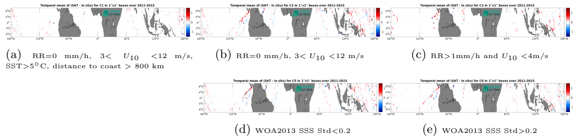
Figure 14: Temporal mean gridded over spatial boxes of size 1^\circ \times 1^\circ of \Delta SSS (Aquarius SSS L3 OR v5 - Monthly - Rain mask (NASA-GSFC) - TSG (LEGOS-DM)) for 5 different subdatasets corresponding to:RR=0 mm/h, 3 < U_{10} < 12 m/s, SST>5°C, distance to coast > 800 km (a), RR=0 mm/h, 3 < U_{10} < 12 m/s (b), RR>1mm/h and U_{10} < 4 m/s (c), WOA2013 SSS Std<0.2 (d), WOA2013 SSS Std>0.2 (e).
