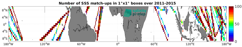
Figure 5: Number of SSS match-ups between TSG (LEGOS-DM) SSS and the Aquarius SSS L3 OR v5 - Monthly - Rain mask (NASA-GSFC) SSS product for the Equatorial Ocean 10N-10S Pi-MEP region over 1^\circ \times 1^\circ boxes and for the full satellite product period.
