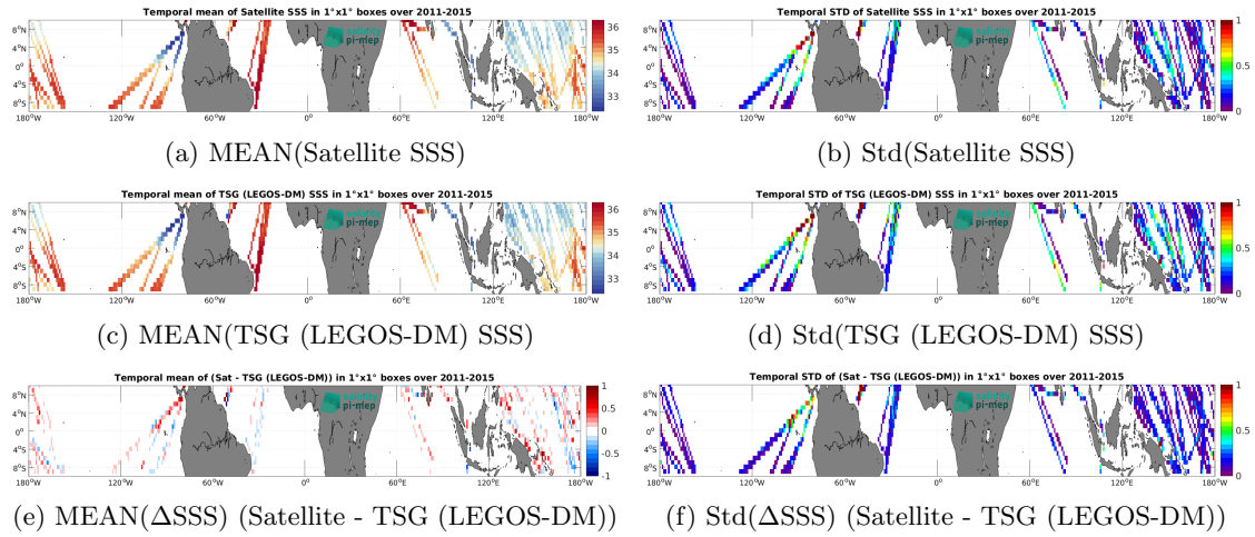
Figure 7: Temporal mean (left) and Std (right) of SSS from Aquarius SSS L3 OR v5 - Monthly - Rain mask (NASA-GSFC) (top), TSG (LEGOS-DM) (middle), and of \Delta SSS (Satellite - TSG (LEGOS-DM)). Only match-up pairs are used to generate these maps.
