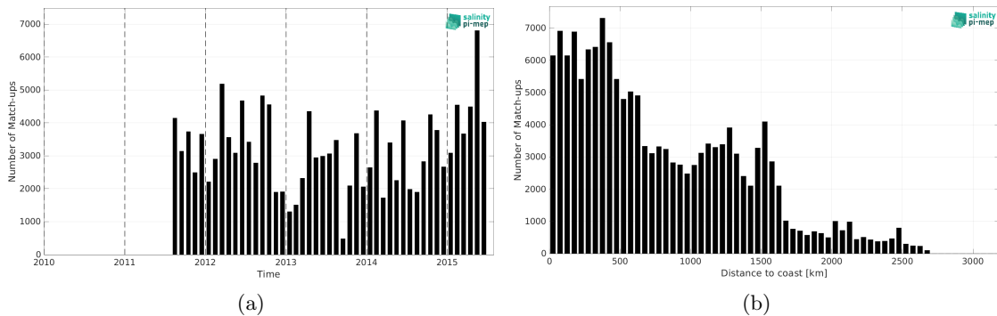
Figure 2: Number of match-ups between TSG (LEGOS-DM) and Aquarius SSS L3 OR v5 - Monthly - Rain mask (NASA-GSFC) SSS as a function of time (a) and as function of the distance to coast (b) over the Equatorial Ocean 10N-10S Pi-MEP region and for the full satellite product period.
