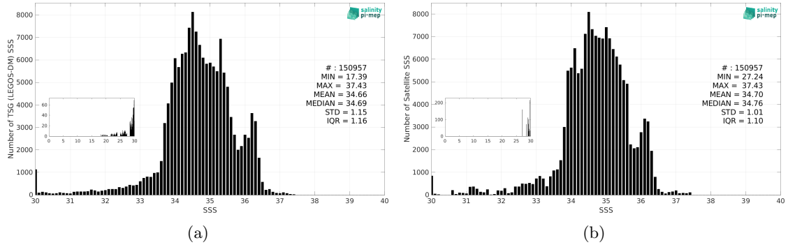
Figure 3: Histograms of SSS from TSG (LEGOS-DM) (a) and Aquarius SSS L3 OR v5 - Monthly - Rain mask (NASA-GSFC) (b) considering all match-up pairs per bins of 0.1 over the Equatorial Ocean 10N-10S Pi-MEP region and for the full satellite product period.
