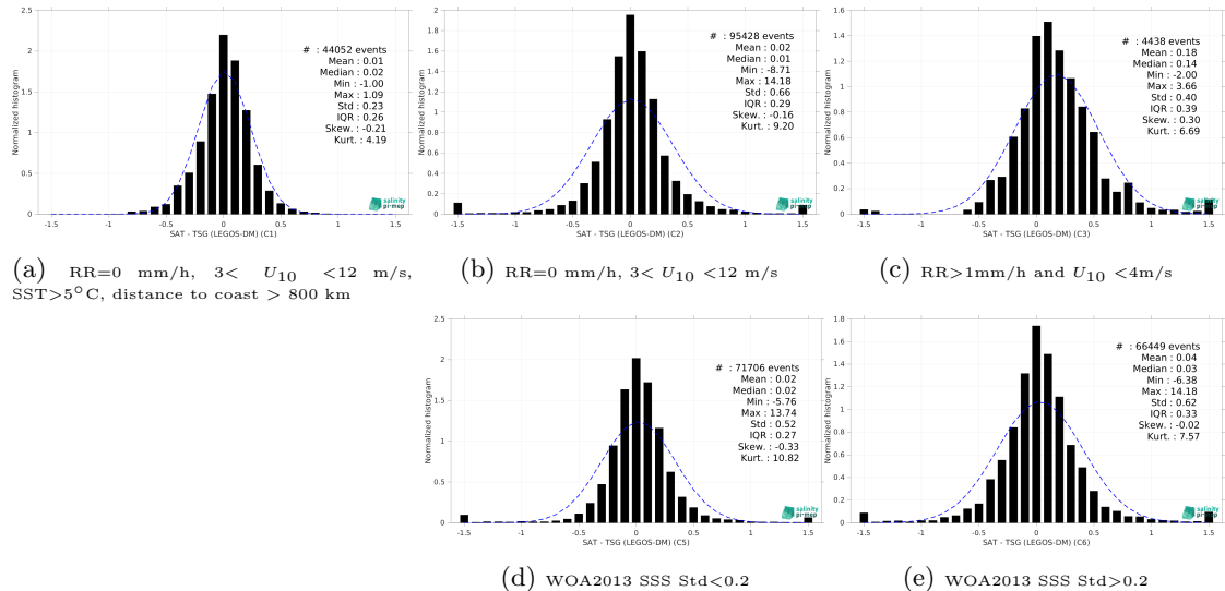
Figure 15: Normalized histogram of \Delta SSS (Aquarius SSS L3 OR v5 - Monthly - Rain mask (NASA-GSFC) - TSG (LEGOS-DM)) for 5 different subdatasets corresponding to: RR=0 mm/h, 3 < U_{10} < 12 m/s, SST>5°C, distance to coast > 800 km (a), RR=0 mm/h, 3 < U_{10} < 12 m/s (b), RR>1mm/h and U_{10} < 4 m/s (c), WOA2013 SSS Std<0.2 (d), WOA2013 SSS Std>0.2 (e).
