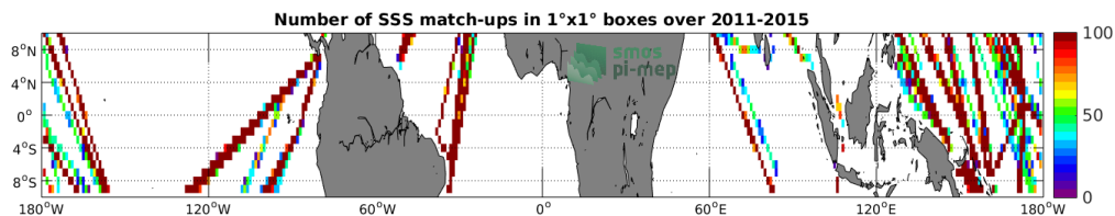
Figure 4: Number of SSS match-ups between TSG-LEGOS-DM SSS and the Aquarius-L3-OR-V5-MONTHLY-RAIN-MASK-1DEG SSS product for the Equatorial Ocean 10N-10S Pi-MEP region over 1^\circ \times 1^\circ boxes and for the full satellite product period.
