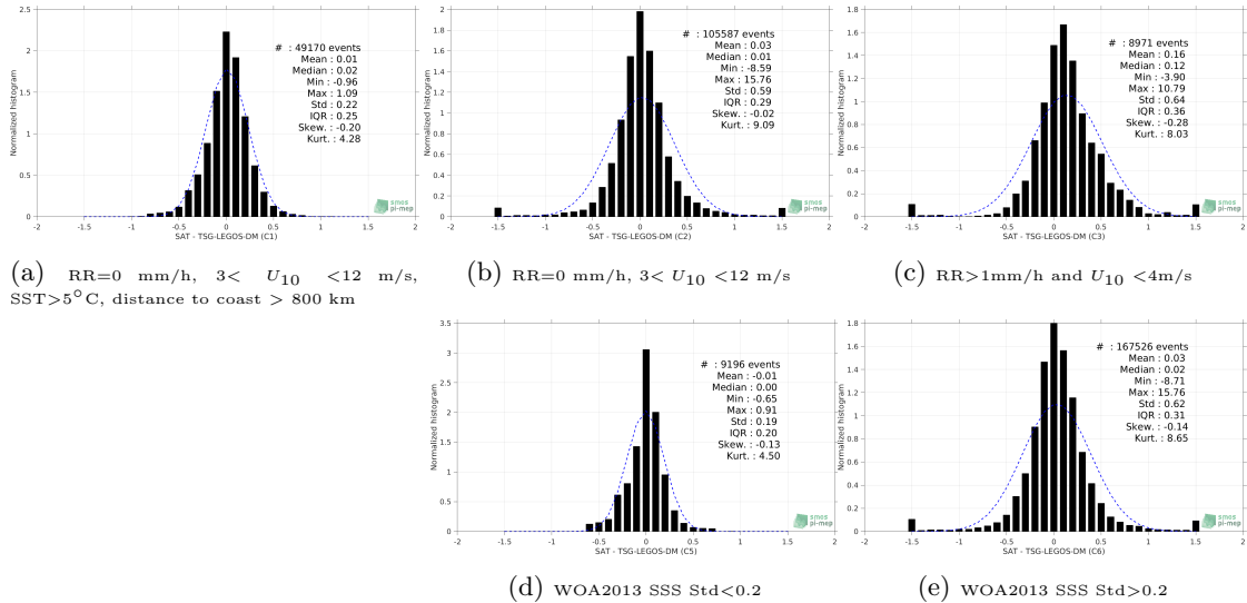
Figure 13: Normalized histogram of \Delta SSS (Aquarius-L3-OR-V5-MONTHLY-RAIN-MASK-1DEG - TSG-LEGOS-DM) for 5 different subdatasets corresponding to: RR=0 mm/h, 3 < U_{10} < 12 m/s, SST >5^\circ\text{C} , distance to coast > 800 km (a), RR=0 mm/h, 3 < U_{10} < 12 m/s (b), RR >1 mm/h and U_{10} < 4 m/s (c), WOA2013 SSS Std <0.2 (d), WOA2013 SSS Std >0.2 (e).
