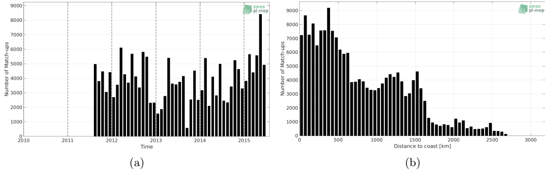
Figure 1: Number of match-ups between TSG-LEGOS-DM and Aquarius-L3-OR-V5-MONTHLY-RAIN-MASK-1DEG SSS as a function of time (a) and as function of the distance to coast (b) over the Equatorial Ocean 10N-10S Pi-MEP region and for the full satellite product period.
