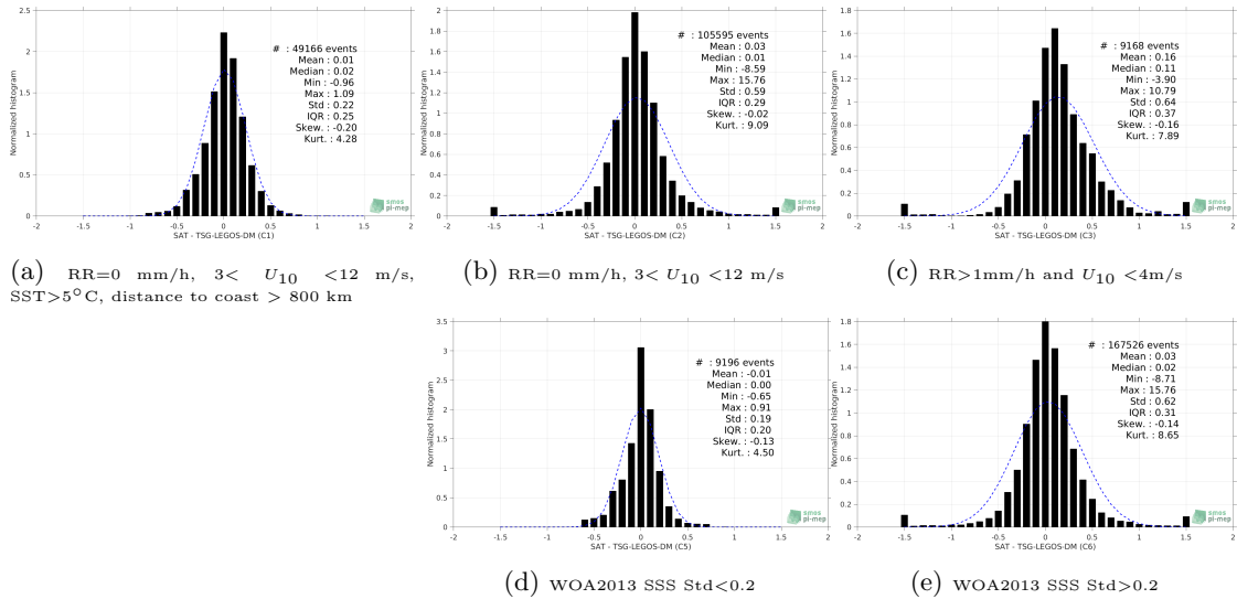
Figure 13: Normalized histogram of \Delta SSS (Aquarius-L3-OR-V5-MONTHLY-RAIN-MASK-1DEG - TSG-LEGOS-DM) for 5 different subdatasets corresponding to: RR=0 mm/h, 3 < U_{10} < 12 m/s, SST >5^\circ\text{C} , distance to coast > 800 km (a), RR=0 mm/h, 3 < U_{10} < 12 m/s (b), RR >1 mm/h and U_{10} < 4 m/s (c), WOA2013 SSS Std <0.2 (d), WOA2013 SSS Std >0.2 (e).
