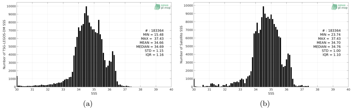
Figure 2: Histograms of SSS from TSG-LEGOS-DM (a) and Aquarius-L3-OR-V5-MONTHLY-RAIN-MASK-1DEG (b) considering all match-up pairs per bins of 0.1 over the Equatorial Ocean 10N-10S Pi-MEP region and for the full satellite product period.
