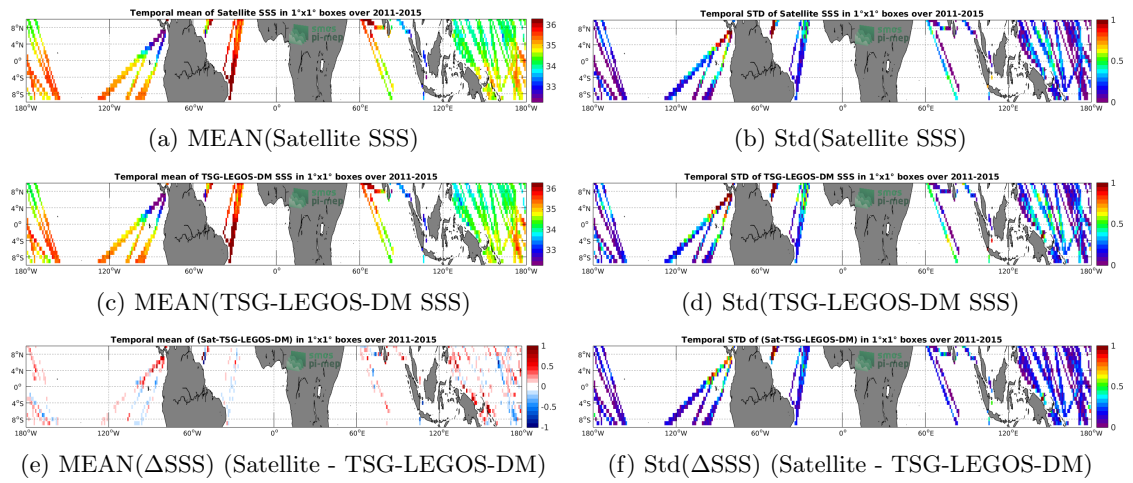
Figure 6: Temporal mean (left) and Std (right) of SSS from Aquarius-L3-OR-V5-MONTHLY-RAIN-MASK-1DEG (top), TSG-LEGOS-DM (middle), and of \Delta SSS (Satellite - TSG-LEGOS-DM). Only match-up pairs are used to generate these maps.
