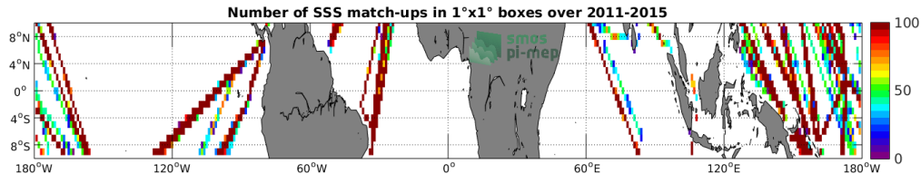
Figure 4: Number of SSS match-ups between TSG-LEGOS-DM SSS and the Aquarius-L3-OR-V5-MONTHLY-RAIN-MASK-1DEG SSS product for the Equatorial Ocean 10N-10S Pi-MEP region over 1°x1° boxes and for the full satellite product period.
