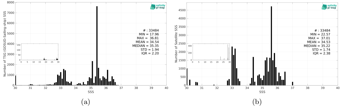
Figure 3: Histograms of SSS from TSG (GOSUD-Sailing-ship) (a) and Aquarius SSS L3 OR v5 - Monthly - Rain mask (NASA-GSFC) (b) considering all match-up pairs per bins of 0.1 over the Equatorial Ocean 10N-10S Pi-MEP region and for the full satellite product period.
