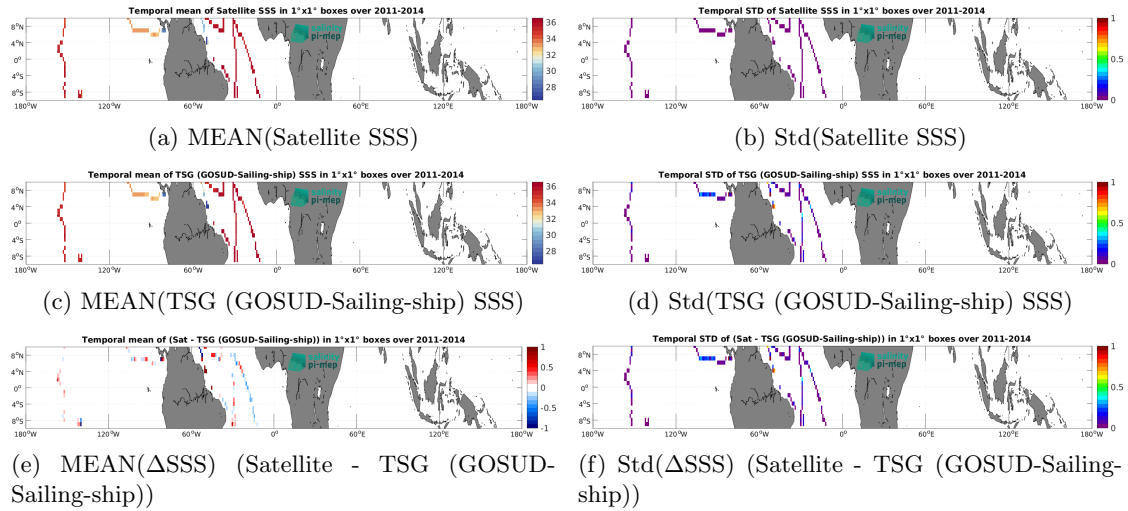
Figure 7: Temporal mean (left) and Std (right) of SSS from Aquarius SSS L3 OR v5 - Monthly - Rain mask (NASA-GSFC) (top), TSG (GOSUD-Sailing-ship) (middle), and of \Delta SSS (Satellite - TSG (GOSUD-Sailing-ship)). Only match-up pairs are used to generate these maps.
