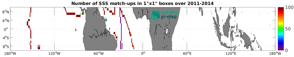
Figure 5: Number of SSS match-ups between TSG (GOSUD-Sailing-ship) SSS and the Aquarius SSS L3 OR v5 - Monthly - Rain mask (NASA-GSFC) SSS product for the Equatorial Ocean 10N-10S Pi-MEP region over 1^\circ \times 1^\circ boxes and for the full satellite product period.
