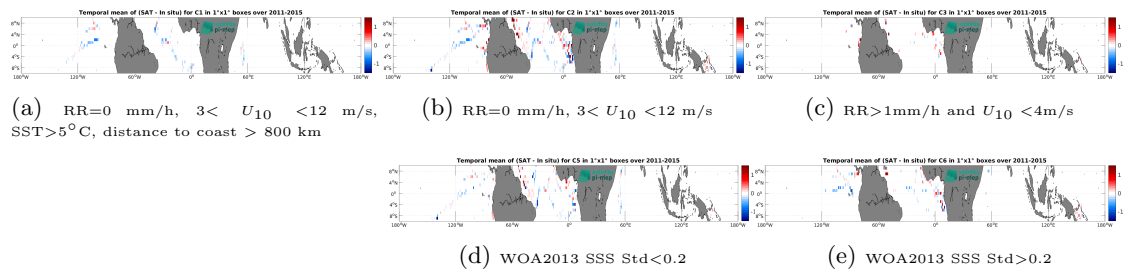
Figure 14: Temporal mean gridded over spatial boxes of size 1^\circ \times 1^\circ of \Delta SSS (Aquarius SSS L3 OR v5 - Monthly - Rain mask (NASA-GSFC) - TSG (GOSUD-Research-vessel)) for 5 different subdatasets corresponding to:RR=0 mm/h, 3 < U_{10} < 12 m/s, SST > 5^\circ\text{C} , distance to coast > 800 km (a), RR=0 mm/h, 3 < U_{10} < 12 m/s (b), RR > 1 mm/h and U_{10} < 4 m/s (c), WOA2013 SSS Std < 0.2 (d), WOA2013 SSS Std > 0.2 (e).
