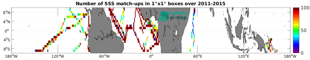
Figure 5: Number of SSS match-ups between TSG (GOSUD-Research-vessel) SSS and the Aquarius SSS L3 OR v5 - Monthly - Rain mask (NASA-GSFC) SSS product for the Equatorial Ocean 10N-10S Pi-MEP region over 1^\circ \times 1^\circ boxes and for the full satellite product period.
