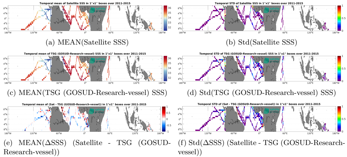
Figure 7: Temporal mean (left) and Std (right) of SSS from Aquarius SSS L3 OR v5 - Monthly - Rain mask (NASA-GSFC) (top), TSG (GOSUD-Research-vessel) (middle), and of \Delta SSS (Satellite - TSG (GOSUD-Research-vessel)). Only match-up pairs are used to generate these maps.
