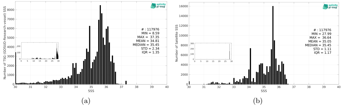
Figure 3: Histograms of SSS from TSG (GOSUD-Research-vessel) (a) and Aquarius SSS L3 OR v5 - Monthly - Rain mask (NASA-GSFC) (b) considering all match-up pairs per bins of 0.1 over the Equatorial Ocean 10N-10S Pi-MEP region and for the full satellite product period.
