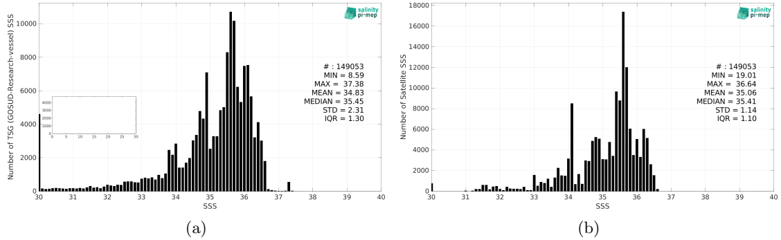
Figure 2: Histograms of SSS from TSG (GOSUD-Research-vessel) (a) and Aquarius SSS L3 OR v5 - Monthly - Rain mask (NASA-GSFC) (b) considering all match-up pairs per bins of 0.1 over the Equatorial Ocean 10N-10S Pi-MEP region and for the full satellite product period.
