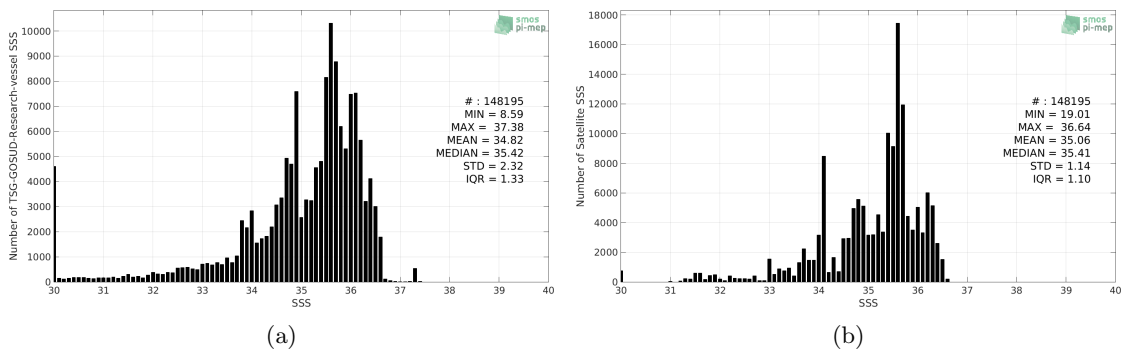
Figure 2: Histograms of SSS from TSG-GOSUD-Research-vessel (a) and Aquarius-L3-OR-V5-MONTHLY-RAIN-MASK-1DEG (b) considering all match-up pairs per bins of 0.1 over the Equatorial Ocean 10N-10S Pi-MEP region and for the full satellite product period.
