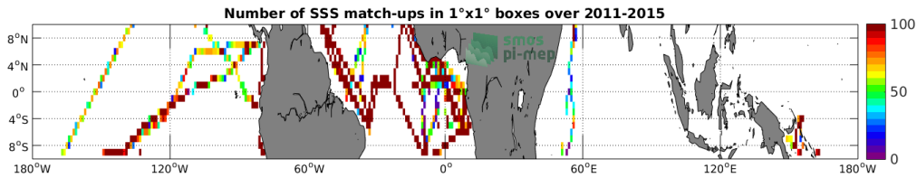
Figure 4: Number of SSS match-ups between TSG-GOSUD-Research-vessel SSS and the Aquarius-L3-OR-V5-MONTHLY-RAIN-MASK-1DEG SSS product for the Equatorial Ocean 10N-10S Pi-MEP region over 1^\circ \times 1^\circ boxes and for the full satellite product period.
