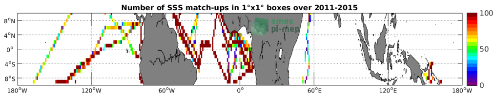
Figure 4: Number of SSS match-ups between TSG-GOSUD-Research-vessel SSS and the Aquarius-L3-OR-V5-MONTHLY-RAIN-MASK-1DEG SSS product for the Equatorial Ocean 10N-10S Pi-MEP region over 1°x1° boxes and for the full satellite product period.
