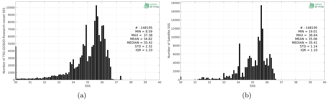
Figure 2: Histograms of SSS from TSG-GOSUD-Research-vessel (a) and Aquarius-L3-OR-V5-MONTHLY-RAIN-MASK-1DEG (b) considering all match-up pairs per bins of 0.1 over the Equatorial Ocean 10N-10S Pi-MEP region and for the full satellite product period.
