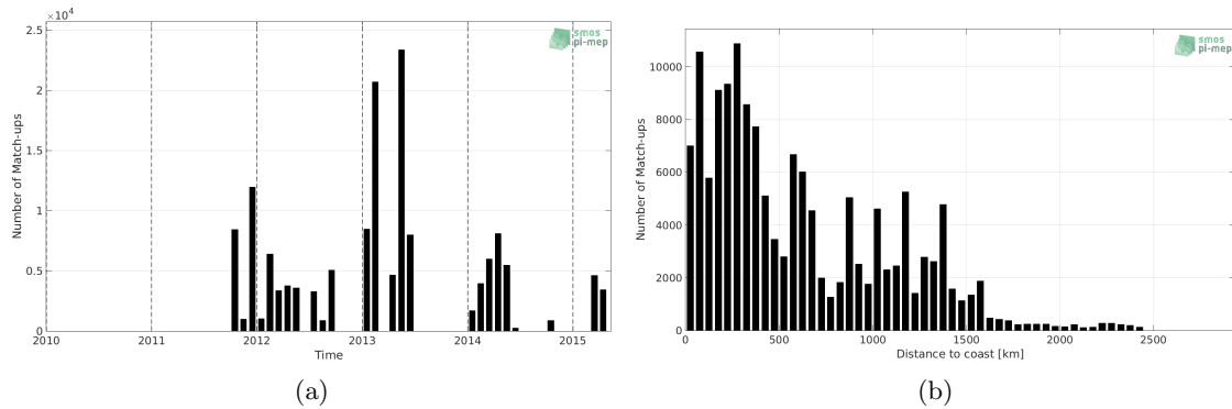
Figure 1: Number of match-ups between TSG-GOSUD-Research-vessel and Aquarius-L3-OR-V5-MONTHLY-RAIN-MASK-1DEG SSS as a function of time (a) and as function of the distance to coast (b) over the Equatorial Ocean 10N-10S Pi-MEP region and for the full satellite product period.
