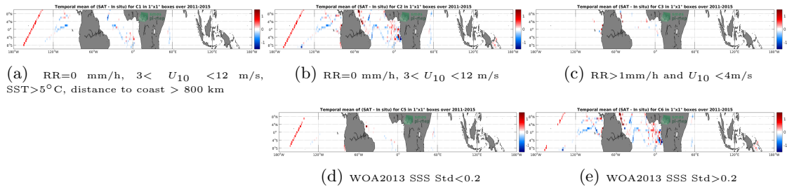
Figure 12: Temporal mean gridded over spatial boxes of size 1^\circ \times 1^\circ of \Delta SSS (Aquarius-L3-OR-V5-MONTHLY-RAIN-MASK-1DEG - TSG-GOSUD-Research-vessel) for 5 different subdatasets corresponding to: RR=0 mm/h, 3 < U_{10} < 12 m/s, SST >5^\circ\text{C} , distance to coast > 800 km (a), RR=0 mm/h, 3 < U_{10} < 12 m/s (b), RR >1 mm/h and U_{10} < 4 m/s (c), WOA2013 SSS Std <0.2 (d), WOA2013 SSS Std >0.2 (e).
