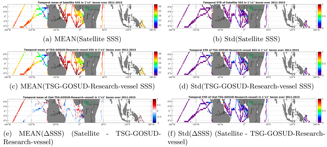
Figure 6: Temporal mean (left) and Std (right) of SSS from Aquarius-L3-OR-V5-MONTHLY-RAIN-MASK-1DEG (top), TSG-GOSUD-Research-vessel (middle), and of \Delta SSS (Satellite - TSG-GOSUD-Research-vessel). Only match-up pairs are used to generate these maps.
