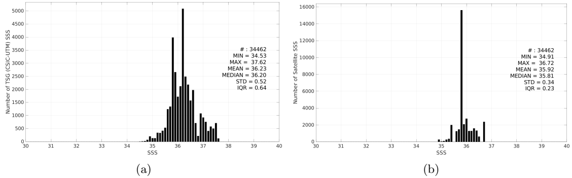
Figure 3: Histograms of SSS from TSG (CSIC-UTM) (a) and Aquarius SSS L3 OR v5 - Monthly - Rain mask (NASA-GSFC) (b) considering all match-up pairs per bins of 0.1 over the Equatorial Ocean 10N-10S Pi-MEP region and for the full satellite product period.
