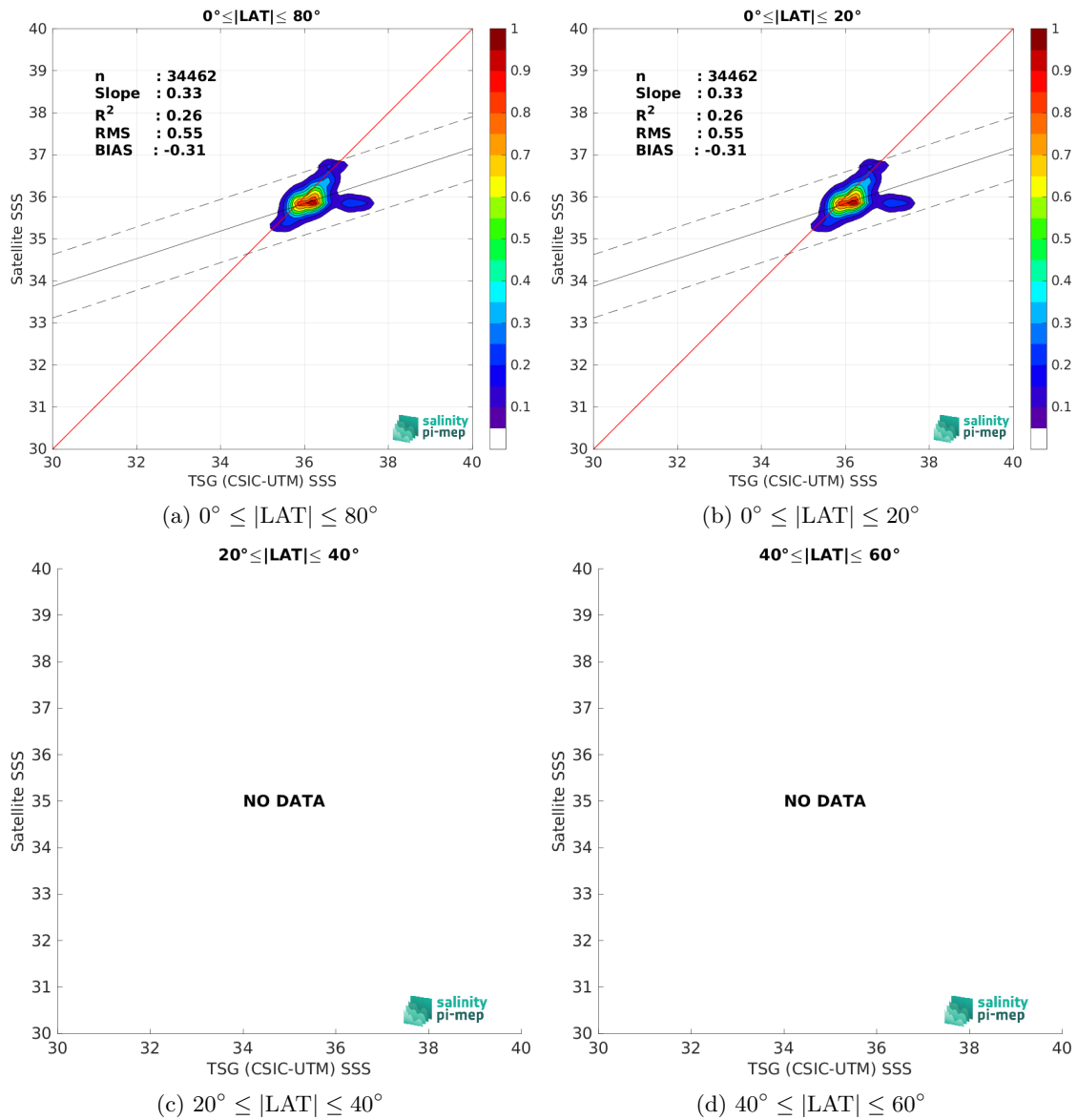
Figure 10: Contour maps of the concentration of Aquarius SSS L3 OR v5 - Monthly - Rain mask (NASA-GSFC) SSS (y-axis) versus TSG (CSIC-UTM) SSS (x-axis) at match-up pairs for different latitude bands. For each plot, the red line shows x=y . The black thin and dashed lines indicate a linear fit through the data cloud and the \pm 95\% confidence levels, respectively. The number match-up pairs n , the slope and R^2 coefficient of the linear fit, the root mean square (RMS) and the mean bias between satellite and in situ data are indicated for each latitude band in each plots.
