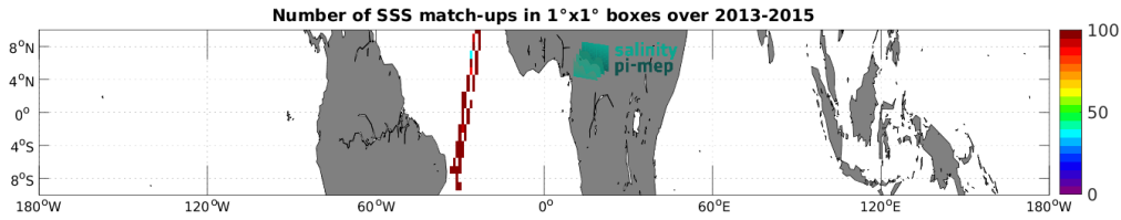
Figure 5: Number of SSS match-ups between TSG (CSIC-UTM) SSS and the Aquarius SSS L3 OR v5 - Monthly - Rain mask (NASA-GSFC) SSS product for the Equatorial Ocean 10N-10S Pi-MEP region over 1^\circ \times 1^\circ boxes and for the full satellite product period.
