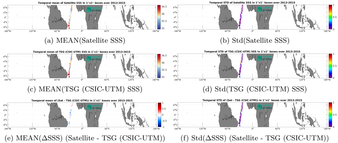
Figure 7: Temporal mean (left) and Std (right) of SSS from Aquarius SSS L3 OR v5 - Monthly - Rain mask (NASA-GSFC) (top), TSG (CSIC-UTM) (middle), and of \Delta SSS (Satellite - TSG (CSIC-UTM)). Only match-up pairs are used to generate these maps.
