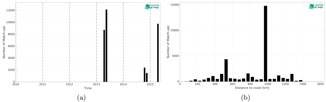
Figure 2: Number of match-ups between TSG (CSIC-UTM) and Aquarius SSS L3 OR v5 - Monthly - Rain mask (NASA-GSFC) SSS as a function of time (a) and as function of the distance to coast (b) over the Equatorial Ocean 10N-10S Pi-MEP region and for the full satellite product period.
