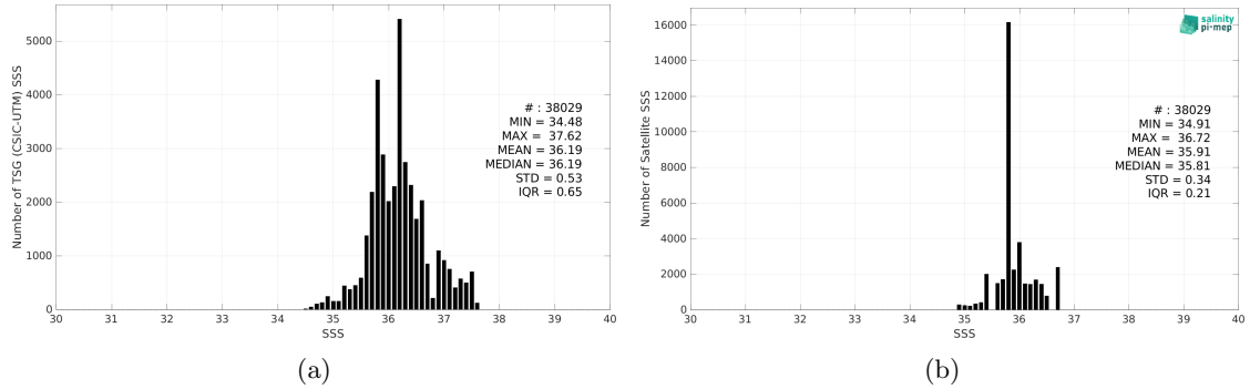
Figure 2: Histograms of SSS from TSG (CSIC-UTM) (a) and Aquarius SSS L3 OR v5 - Monthly - Rain mask (NASA-GSFC) (b) considering all match-up pairs per bins of 0.1 over the Equatorial Ocean 10N-10S Pi-MEP region and for the full satellite product period.
