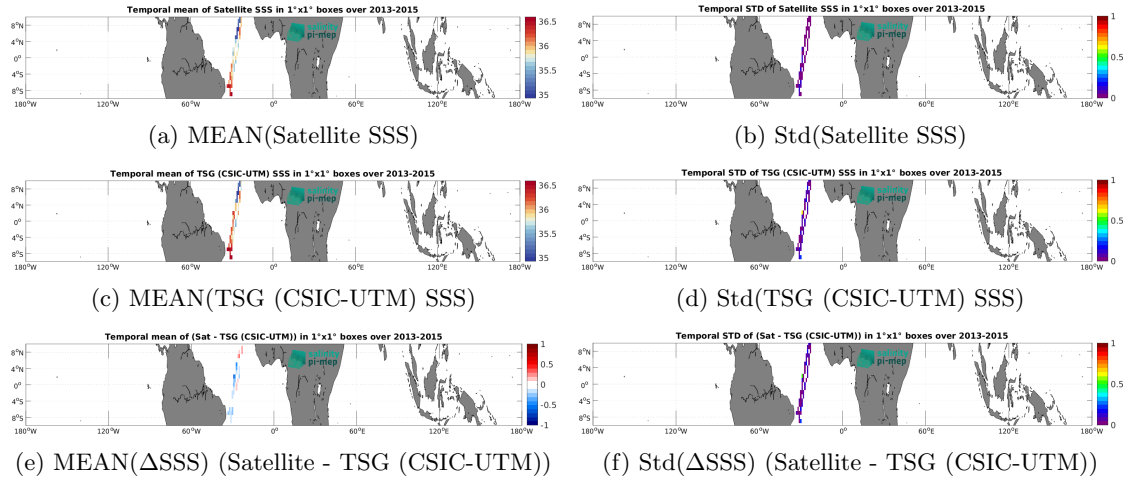
Figure 6: Temporal mean (left) and Std (right) of SSS from Aquarius SSS L3 OR v5 - Monthly - Rain mask (NASA-GSFC) (top), TSG (CSIC-UTM) (middle), and of \Delta SSS (Satellite - TSG (CSIC-UTM)). Only match-up pairs are used to generate these maps.
