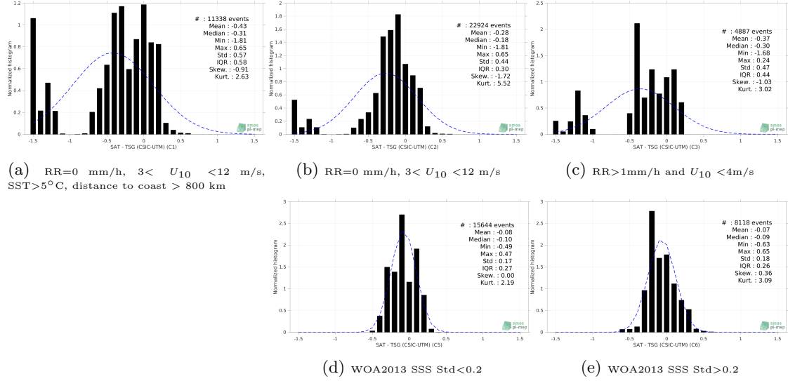
Figure 13: Normalized histogram of \Delta\text{SSS} (Aquarius SSS L3 OR v5 - Monthly - Rain mask (NASA-GSFC) - TSG (CSIC-UTM)) for 5 different subdatasets corresponding to: RR=0 mm/h, 3 < U_{10} < 12 m/s, SST>5°C, distance to coast > 800 km (a), RR=0 mm/h, 3 < U_{10} < 12 m/s (b), RR>1mm/h and U_{10} < 4 m/s (c), WOA2013 SSS Std<0.2 (d), WOA2013 SSS Std>0.2 (e).
