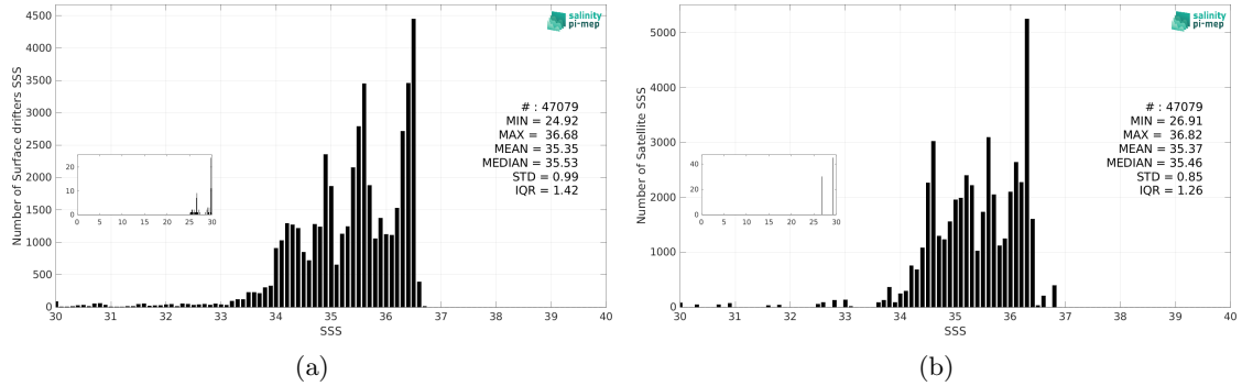
Figure 3: Histograms of SSS from Surface drifters (a) and Aquarius SSS L3 OR v5 - Monthly - Rain mask (NASA-GSFC) (b) considering all match-up pairs per bins of 0.1 over the Equatorial Ocean 10N-10S Pi-MEP region and for the full satellite product period.
