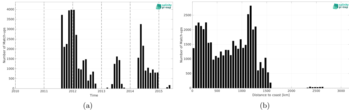
Figure 2: Number of match-ups between Surface drifters and Aquarius SSS L3 OR v5 - Monthly - Rain mask (NASA-GSFC) SSS as a function of time (a) and as function of the distance to coast (b) over the Equatorial Ocean 10N-10S Pi-MEP region and for the full satellite product period.
