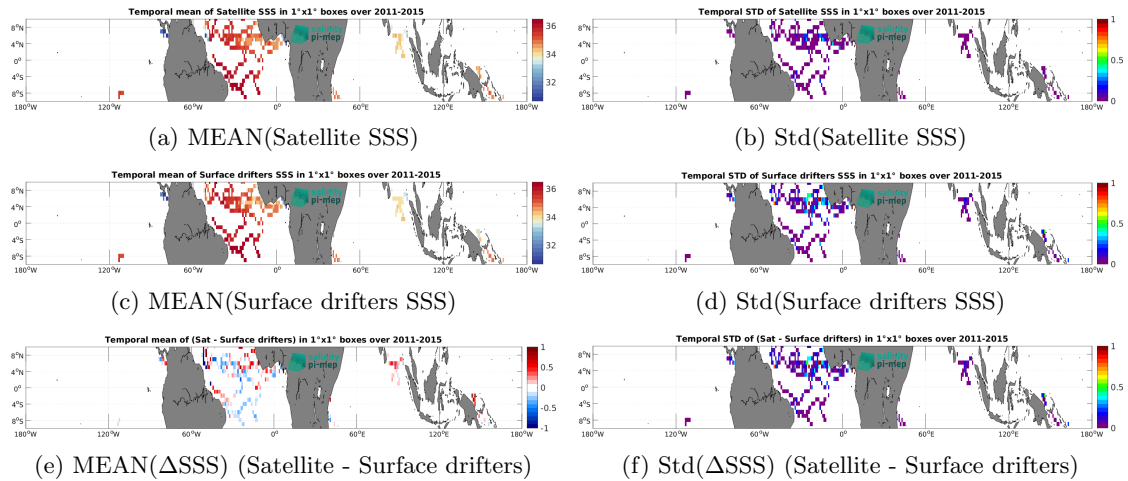
Figure 6: Temporal mean (left) and Std (right) of SSS from Aquarius SSS L3 OR v5 - Monthly - Rain mask (NASA-GSFC) (top), Surface drifters (middle), and of \Delta SSS (Satellite - Surface drifters). Only match-up pairs are used to generate these maps.
