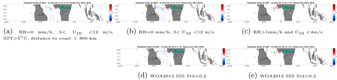
Figure 13: Temporal mean gridded over spatial boxes of size 1^\circ \times 1^\circ of \Delta SSS (Aquarius SSS L3 OR v5 - Monthly - Rain mask (NASA-GSFC) - Surface drifters) for 5 different subdatasets corresponding to: RR=0 mm/h, 3 < U_{10} < 12 m/s, SST >5^\circ C, distance to coast > 800 km (a), RR=0 mm/h, 3 < U_{10} < 12 m/s (b), RR >1 mm/h and U_{10} < 4 m/s (c), WOA2013 SSS Std <0.2 (d), WOA2013 SSS Std >0.2 (e).
