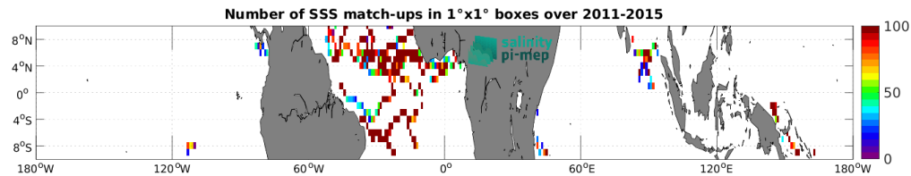
Figure 4: Number of SSS match-ups between Surface drifters SSS and the Aquarius SSS L3 OR v5 - Monthly - Rain mask (NASA-GSFC) SSS product for the Equatorial Ocean 10N-10S Pi-MEP region over 1^\circ \times 1^\circ boxes and for the full satellite product period.
