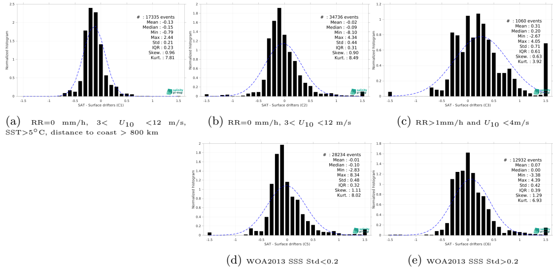
Figure 14: Normalized histogram of \Delta SSS (Aquarius SSS L3 OR v5 - Monthly - Rain mask (NASA-GSFC) - Surface drifters) for 5 different subdatasets corresponding to: RR=0 mm/h, 3 < U_{10} < 12 m/s, SST >5^\circ C, distance to coast > 800 km (a), RR=0 mm/h, 3 < U_{10} < 12 m/s (b), RR >1 mm/h and U_{10} < 4 m/s (c), WOA2013 SSS Std <0.2 (d), WOA2013 SSS Std >0.2 (e).
