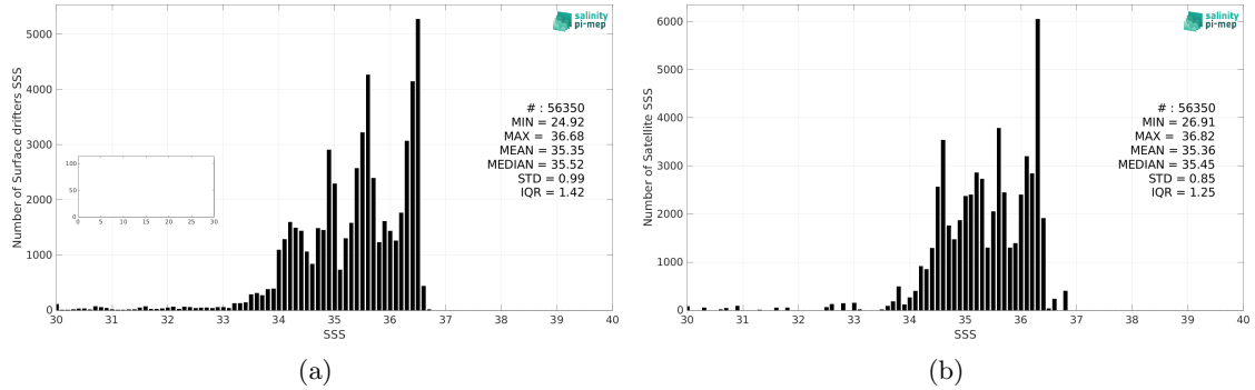
Figure 2: Histograms of SSS from Surface drifters (a) and Aquarius SSS L3 OR v5 - Monthly - Rain mask (NASA-GSFC) (b) considering all match-up pairs per bins of 0.1 over the Equatorial Ocean 10N-10S Pi-MEP region and for the full satellite product period.
