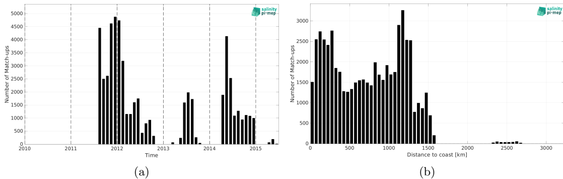
Figure 1: Number of match-ups between Surface drifters and Aquarius SSS L3 OR v5 - Monthly - Rain mask (NASA-GSFC) SSS as a function of time (a) and as function of the distance to coast (b) over the Equatorial Ocean 10N-10S Pi-MEP region and for the full satellite product period.
