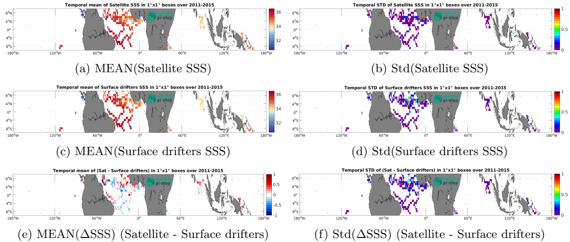
Figure 5: Temporal mean (left) and Std (right) of SSS from Aquarius SSS L3 OR v5 - Monthly - Rain mask (NASA-GSFC) (top), Surface drifters (middle), and of \Delta SSS (Satellite - Surface drifters). Only match-up pairs are used to generate these maps.
