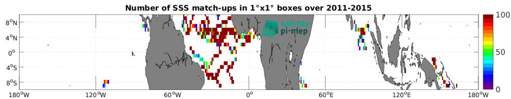
Figure 3: Number of SSS match-ups between Surface drifters SSS and the Aquarius SSS L3 OR v5 - Monthly - Rain mask (NASA-GSFC) SSS product for the Equatorial Ocean 10N-10S Pi-MEP region over 1^\circ \times 1^\circ boxes and for the full satellite product period.
