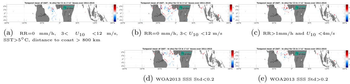
Figure 11: Temporal mean gridded over spatial boxes of size 1^\circ \times 1^\circ of \Delta SSS (Aquarius SSS L3 OR v5 - Monthly - Rain mask (NASA-GSFC) - Surface drifters) for 5 different subdatasets corresponding to: RR=0 mm/h, 3 < U_{10} < 12 m/s, SST >5^\circ C, distance to coast > 800 km (a), RR=0 mm/h, 3 < U_{10} < 12 m/s (b), RR >1 mm/h and U_{10} < 4 m/s (c), WOA2013 SSS Std <0.2 (d), WOA2013 SSS Std >0.2 (e).
