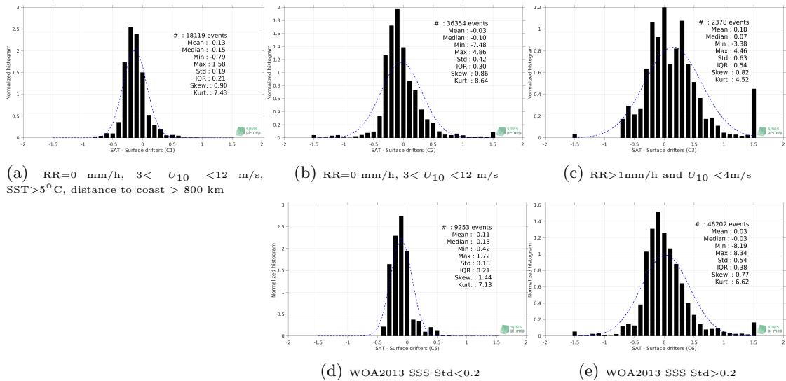
Figure 12: Normalized histogram of \Delta SSS (Aquarius-L3-OR-V5-MONTHLY-RAIN-MASK-1DEG - Surface drifters) for 5 different subdatasets corresponding to: RR=0 mm/h, 3 < U_{10} < 12 m/s, SST >5^\circ\text{C} , distance to coast > 800 km (a), RR=0 mm/h, 3 < U_{10} < 12 m/s (b), RR >1 mm/h and U_{10} < 4 m/s (c), WOA2013 SSS Std <0.2 (d), WOA2013 SSS Std >0.2 (e).
