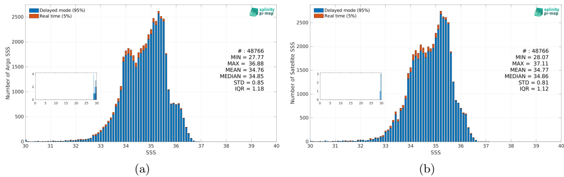
Figure 3: Histograms of SSS from Argo (a) and Aquarius SSS L3 OR v5 - Monthly - Rain mask (NASA-GSFC) (b) considering all match-up pairs per bins of 0.1 over the Equatorial Ocean 10N-10S Pi-MEP region and for the full satellite product period.
