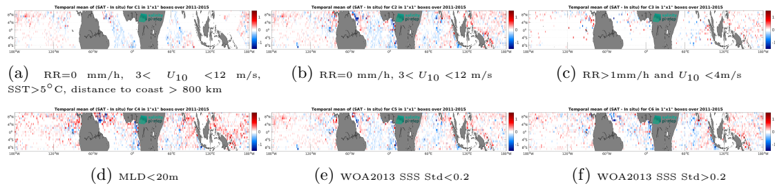
Figure 14: Temporal mean gridded over spatial boxes of size 1^\circ \times 1^\circ of \Delta SSS (Aquarius SSS L3 OR v5 - Monthly - Rain mask (NASA-GSFC) - Argo) for 6 different subdatasets corresponding to:RR=0 mm/h, 3 < U_{10} < 12 m/s, SST >5^\circ C, distance to coast > 800 km (a), RR=0 mm/h, 3 < U_{10} < 12 m/s (b), RR >1 mm/h and U_{10} < 4 m/s (c),MLD <20 m (d),WOA2013 SSS Std <0.2 (e),WOA2013 SSS Std >0.2 (f).
