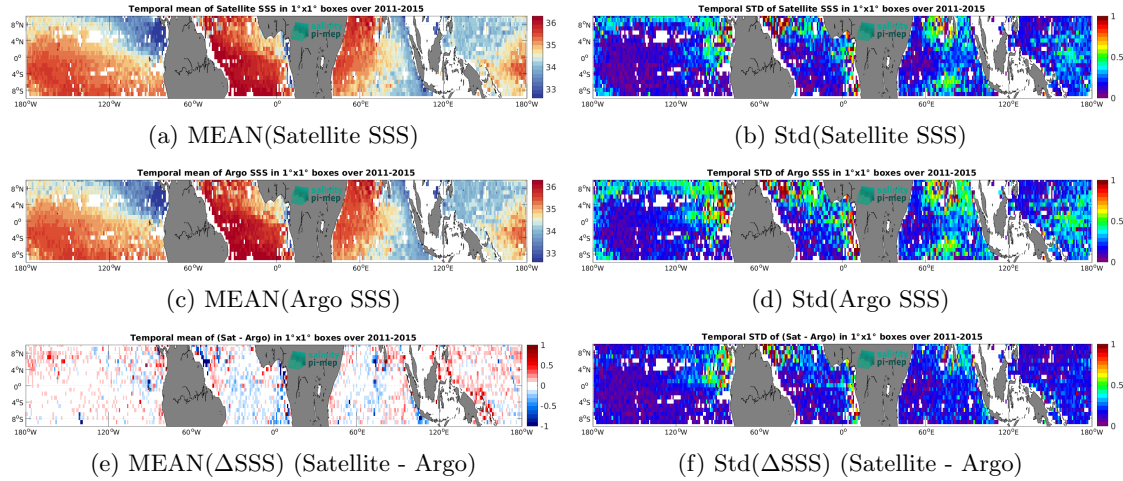
Figure 7: Temporal mean (left) and Std (right) of SSS from Aquarius SSS L3 OR v5 - Monthly - Rain mask (NASA-GSFC) (top), Argo (middle), and of \Delta SSS (Satellite - Argo). Only match-up pairs are used to generate these maps.
