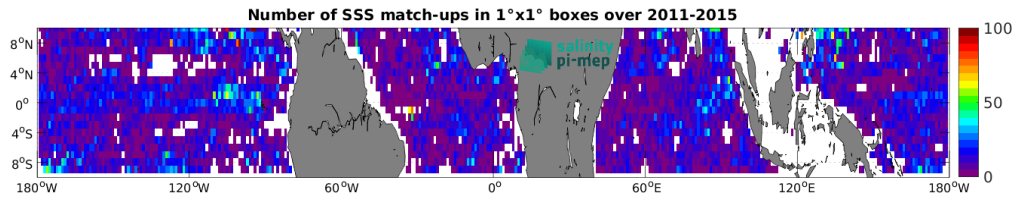
Figure 5: Number of SSS match-ups between Argo SSS and the Aquarius SSS L3 OR v5 - Monthly - Rain mask (NASA-GSFC) SSS product for the Equatorial Ocean 10N-10S Pi-MEP region over 1^\circ \times 1^\circ boxes and for the full satellite product period.
