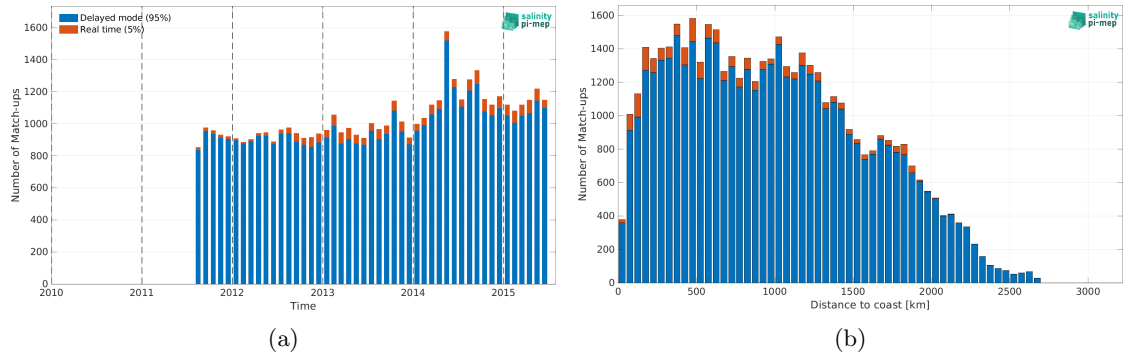
Figure 2: Number of match-ups between Argo and Aquarius SSS L3 OR v5 - Monthly - Rain mask (NASA-GSFC) SSS as a function of time (a) and as function of the distance to coast (b) over the Equatorial Ocean 10N-10S Pi-MEP region and for the full satellite product period.
