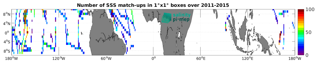
Figure 5: Number of SSS match-ups between TSG (SAMOS) SSS and the Aquarius SSS L3 CAP v5 - 7-Day running (JPL) SSS product for the Equatorial Ocean 10N-10S Pi-MEP region over 1^\circ \times 1^\circ boxes and for the full satellite product period.
