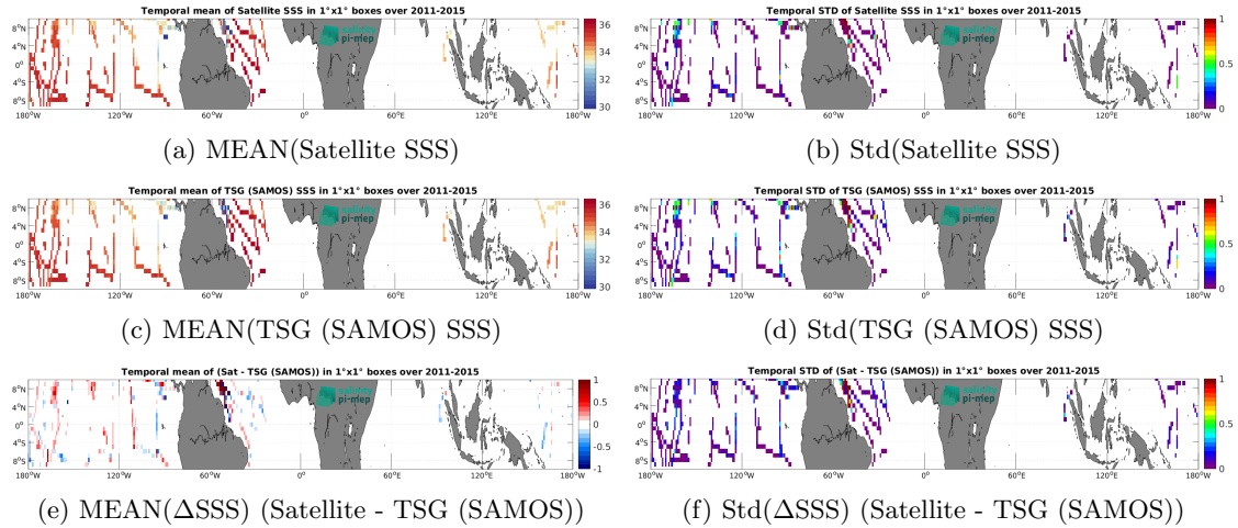
Figure 7: Temporal mean (left) and Std (right) of SSS from Aquarius SSS L3 CAP v5 - 7-Day running (JPL) (top), TSG (SAMOS) (middle), and of \Delta SSS (Satellite - TSG (SAMOS)). Only match-up pairs are used to generate these maps.
