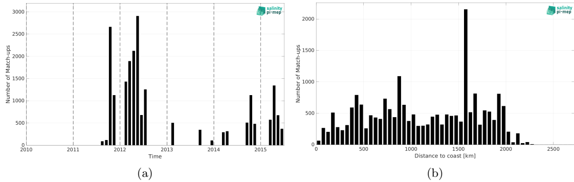
Figure 2: Number of match-ups between TSG (SAMOS) and Aquarius SSS L3 CAP v5 - 7-Day running (JPL) SSS as a function of time (a) and as function of the distance to coast (b) over the Equatorial Ocean 10N-10S Pi-MEP region and for the full satellite product period.
