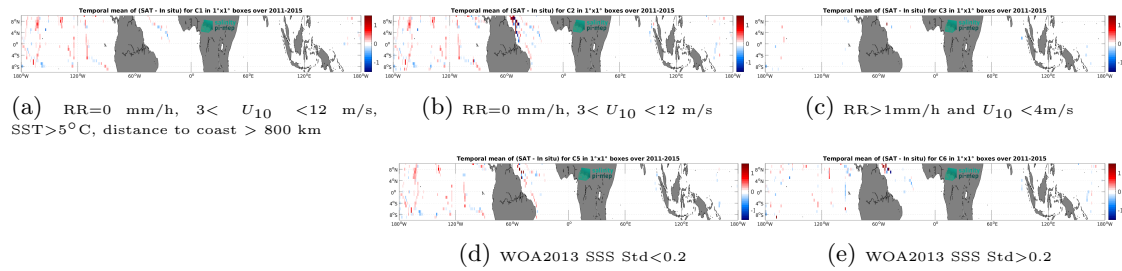
Figure 14: Temporal mean gridded over spatial boxes of size 1^\circ \times 1^\circ of \Delta SSS (Aquarius SSS L3 CAP v5 - 7-Day running (JPL) - TSG (SAMOS)) for 5 different subdatasets corresponding to: RR=0 mm/h, 3 < U_{10} < 12 m/s, SST>5°C, distance to coast > 800 km (a), RR=0 mm/h, 3 < U_{10} < 12 m/s (b), RR>1mm/h and U_{10} < 4 m/s (c), WOA2013 SSS Std<0.2 (d), WOA2013 SSS Std>0.2 (e).
