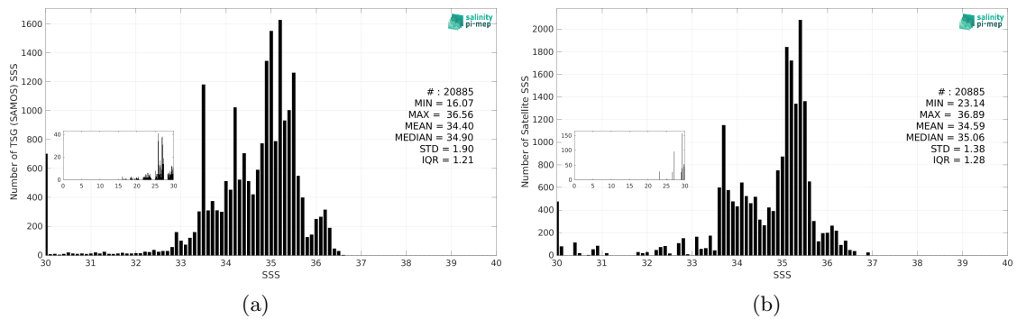
Figure 3: Histograms of SSS from TSG (SAMOS) (a) and Aquarius SSS L3 CAP v5 - 7-Day running (JPL) (b) considering all match-up pairs per bins of 0.1 over the Equatorial Ocean 10N-10S Pi-MEP region and for the full satellite product period.
