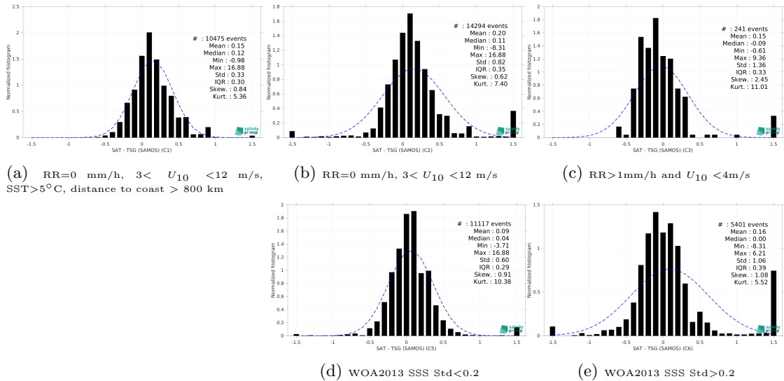
Figure 15: Normalized histogram of \Delta SSS (Aquarius SSS L3 CAP v5 - 7-Day running (JPL) - TSG (SAMOS)) for 5 different subdatasets corresponding to: RR=0 mm/h, 3 < U_{10} < 12 m/s, SST >5^\circ C, distance to coast > 800 km (a), RR=0 mm/h, 3 < U_{10} < 12 m/s (b), RR >1 mm/h and U_{10} < 4 m/s (c), WOA2013 SSS Std <0.2 (d), WOA2013 SSS Std >0.2 (e).
