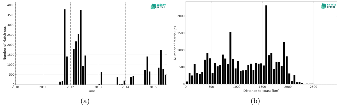
Figure 1: Number of match-ups between TSG (SAMOS) and Aquarius SSS L3 CAP v5 - 7-Day running (JPL) SSS as a function of time (a) and as function of the distance to coast (b) over the Equatorial Ocean 10N-10S Pi-MEP region and for the full satellite product period.
