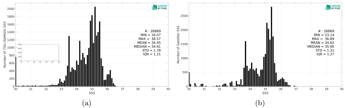
Figure 2: Histograms of SSS from TSG (SAMOS) (a) and Aquarius SSS L3 CAP v5 - 7-Day running (JPL) (b) considering all match-up pairs per bins of 0.1 over the Equatorial Ocean 10N-10S Pi-MEP region and for the full satellite product period.
