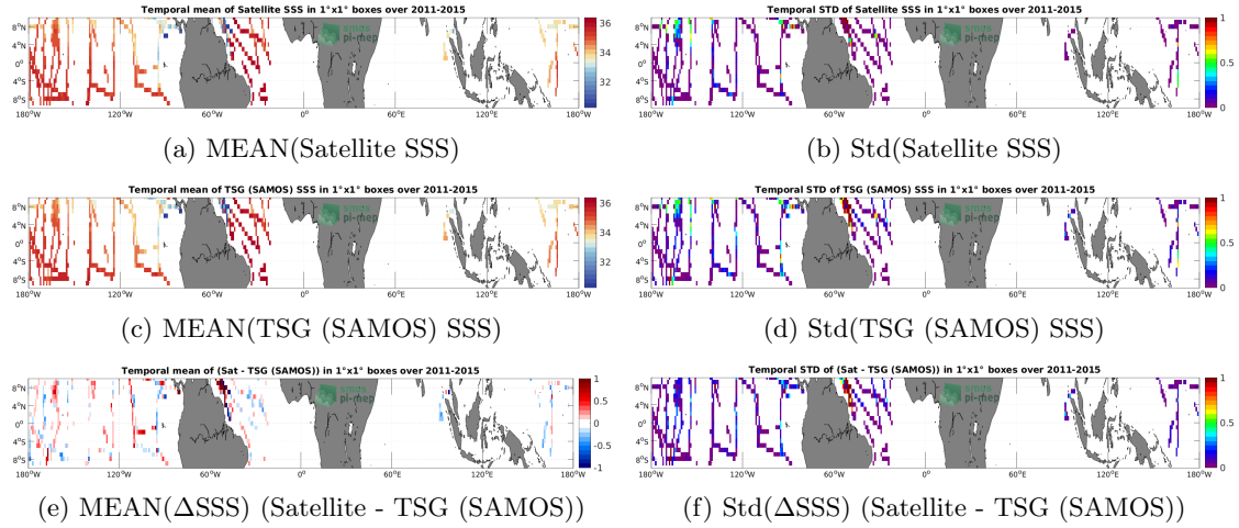
Figure 6: Temporal mean (left) and Std (right) of SSS from Aquarius SSS L3 CAP v5 - 7-Day running (JPL) (top), TSG (SAMOS) ( in situ ) dataset (middle), and of \Delta SSS (Satellite - TSG (SAMOS)). Only match-up pairs are used to generate these maps.
