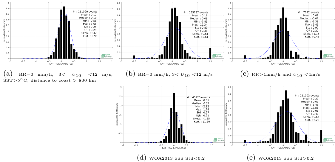
Figure 13: Normalized histogram of \Delta SSS (Aquarius-L3-JPL-V5-7DAY-RUNNING - TSG-SAMOS) for 5 different subdatasets corresponding to: RR=0 mm/h, 3 < U_{10} < 12 m/s, SST > 5^\circ\text{C} , distance to coast > 800 km (a), RR=0 mm/h, 3 < U_{10} < 12 m/s (b), RR > 1 mm/h and U_{10} < 4 m/s (c), WOA2013 SSS Std < 0.2 (d), WOA2013 SSS Std > 0.2 (e).
