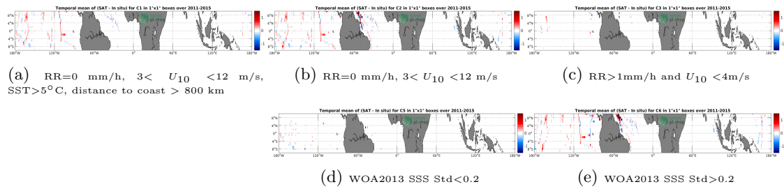
Figure 12: Temporal mean gridded over spatial boxes of size 1^\circ \times 1^\circ of \Delta SSS (Aquarius-L3-JPL-V5-7DAY-RUNNING - TSG-SAMOS) for 5 different subdatasets corresponding to:RR=0 mm/h, 3 < U_{10} < 12 m/s, SST > 5^\circ\text{C} , distance to coast > 800 km (a), RR=0 mm/h, 3 < U_{10} < 12 m/s (b), RR > 1 mm/h and U_{10} < 4 m/s (c), WOA2013 SSS Std < 0.2 (d), WOA2013 SSS Std > 0.2 (e).
