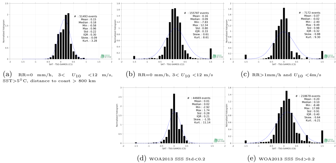
Figure 13: Normalized histogram of \Delta SSS (Aquarius-L3-JPL-V5-7DAY-RUNNING - TSG-SAMOS) for 5 different subdatasets corresponding to: RR=0 mm/h, 3 < U_{10} < 12 m/s, SST >5^\circ\text{C} , distance to coast > 800 km (a), RR=0 mm/h, 3 < U_{10} < 12 m/s (b), RR >1 mm/h and U_{10} < 4 m/s (c), WOA2013 SSS Std <0.2 (d), WOA2013 SSS Std >0.2 (e).
