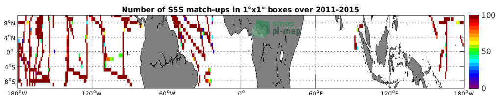
Figure 4: Number of SSS match-ups between TSG-SAMOS SSS and the Aquarius-L3-JPL-V5-7DAY-RUNNING SSS product for the Equatorial Ocean 10N-10S Pi-MEP region over 1^\circ \times 1^\circ boxes and for the full satellite product period.
