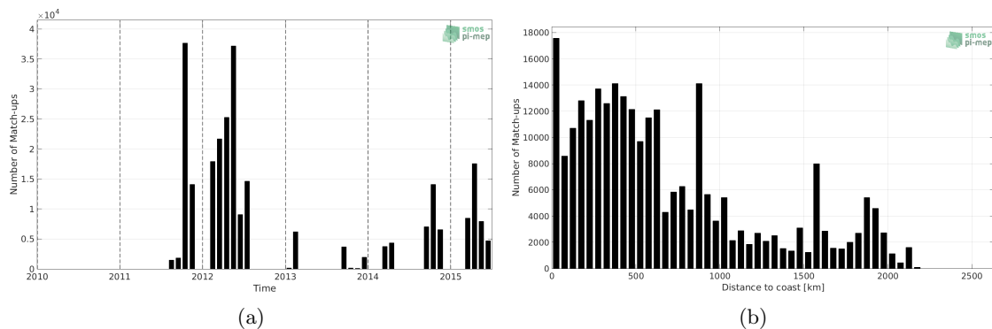
Figure 1: Number of match-ups between TSG-SAMOS and Aquarius-L3-JPL-V5-7DAY-RUNNING SSS as a function of time (a) and as function of the distance to coast (b) over the Equatorial Ocean 10N-10S Pi-MEP region and for the full satellite product period.
