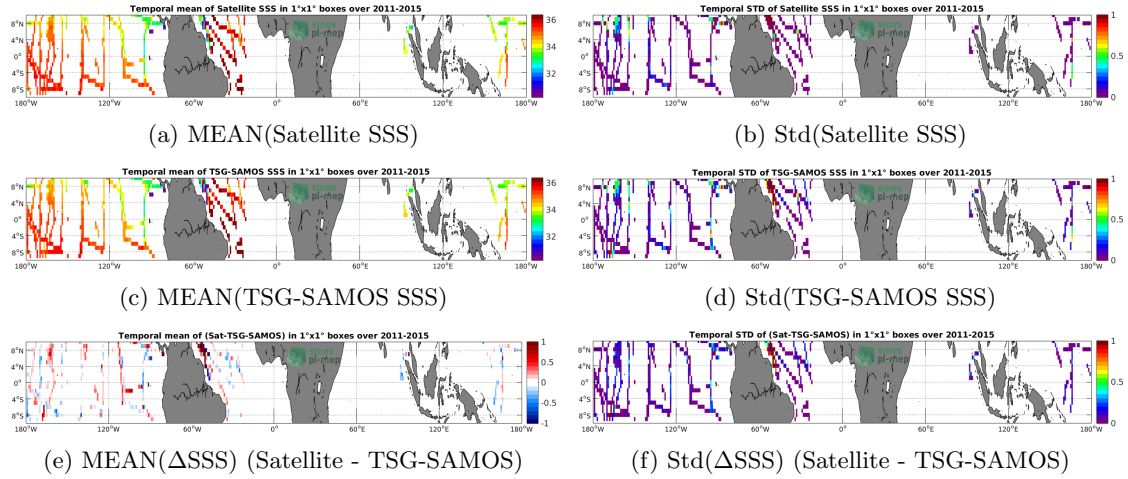
Figure 6: Temporal mean (left) and Std (right) of SSS from Aquarius-L3-JPL-V5-7DAY-RUNNING (top), TSG-SAMOS (middle), and of \Delta SSS (Satellite - TSG-SAMOS). Only match-up pairs are used to generate these maps.
