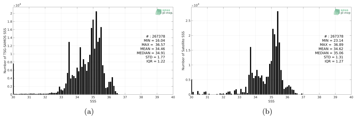
Figure 2: Histograms of SSS from TSG-SAMOS (a) and Aquarius-L3-JPL-V5-7DAY-RUNNING (b) considering all match-up pairs per bins of 0.1 over the Equatorial Ocean 10N-10S Pi-MEP region and for the full satellite product period.
