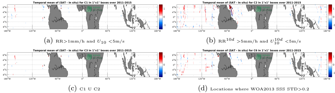
Figure 12: Temporal mean gridded over spatial boxes of size 1^\circ \times 1^\circ of \Delta SSS (Aquarius-L3-JPL-V5-7DAY-RUNNING - TSG-SAMOS) for 4 different subdatasets corresponding to: RR > 1\text{mm/h} and U_{10} < 5\text{m/s} (a), RR^{10d} > 5\text{mm/h} and U_{10}^{10d} < 5\text{m/s} (b), C1 U C2 (c), Locations where WOA2013 SSS STD > 0.2 (d).
