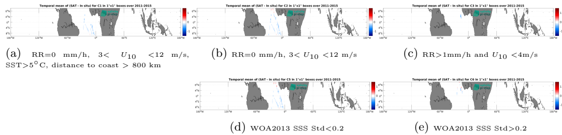
Figure 12: Temporal mean gridded over spatial boxes of size 1^\circ \times 1^\circ of \Delta\text{SSS} (Aquarius SSS L3 CAP v5 - 7-Day running (JPL) - TSG (Polarstern)) for 5 different subdatasets corresponding to: RR=0 mm/h, 3 < U_{10} < 12 m/s, SST >5^\circ\text{C} , distance to coast > 800 km (a), RR=0 mm/h, 3 < U_{10} < 12 m/s (b), RR >1 mm/h and U_{10} < 4 m/s (c), WOA2013 SSS Std <0.2 (d), WOA2013 SSS Std >0.2 (e).
