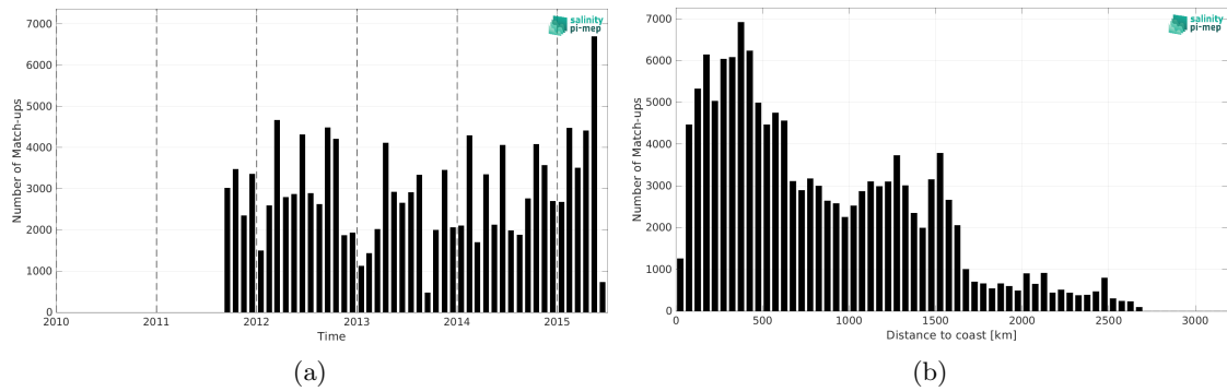
Figure 2: Number of match-ups between TSG (LEGOS-DM) and Aquarius SSS L3 CAP v5 - 7-Day running (JPL) SSS as a function of time (a) and as function of the distance to coast (b) over the Equatorial Ocean 10N-10S Pi-MEP region and for the full satellite product period.
