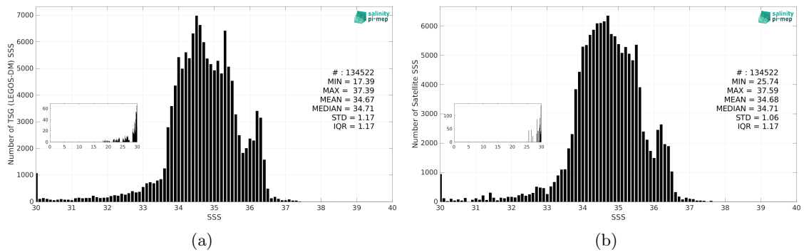
Figure 3: Histograms of SSS from TSG (LEGOS-DM) (a) and Aquarius SSS L3 CAP v5 - 7-Day running (JPL) (b) considering all match-up pairs per bins of 0.1 over the Equatorial Ocean 10N-10S Pi-MEP region and for the full satellite product period.
