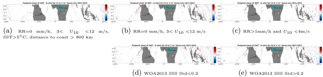
Figure 14: Temporal mean gridded over spatial boxes of size 1^\circ \times 1^\circ of \Delta\text{SSS} (Aquarius SSS L3 CAP v5 - 7-Day running (JPL) - TSG (LEGOS-DM)) for 5 different subdatasets corresponding to: RR=0 mm/h, 3 < U_{10} < 12 m/s, SST>5°C, distance to coast > 800 km (a), RR=0 mm/h, 3 < U_{10} < 12 m/s (b), RR>1mm/h and U_{10} < 4 m/s (c), WOA2013 SSS Std<0.2 (d), WOA2013 SSS Std>0.2 (e).
