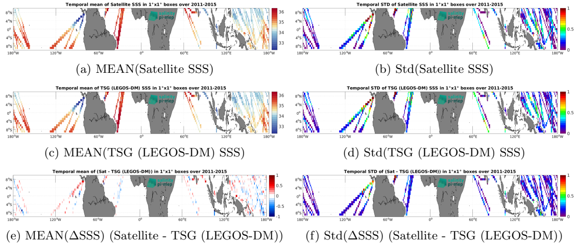
Figure 7: Temporal mean (left) and Std (right) of SSS from Aquarius SSS L3 CAP v5 - 7-Day running (JPL) (top), TSG (LEGOS-DM) (middle), and of \Delta SSS (Satellite - TSG (LEGOS-DM)). Only match-up pairs are used to generate these maps.
