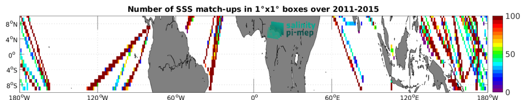
Figure 5: Number of SSS match-ups between TSG (LEGOS-DM) SSS and the Aquarius SSS L3 CAP v5 - 7-Day running (JPL) SSS product for the Equatorial Ocean 10N-10S Pi-MEP region over 1^\circ \times 1^\circ boxes and for the full satellite product period.
