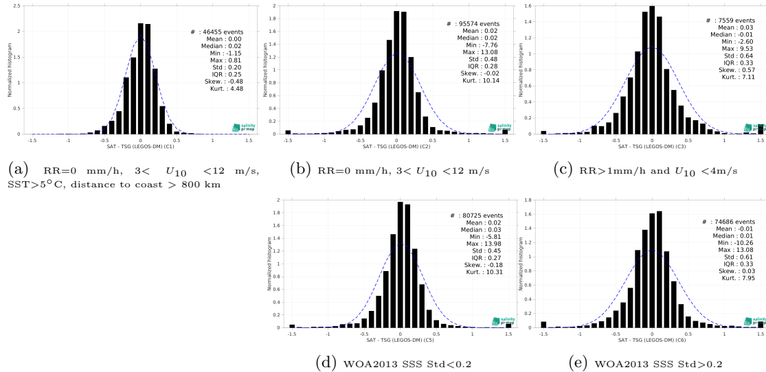
Figure 13: Normalized histogram of \Delta SSS (Aquarius SSS L3 CAP v5 - 7-Day running (JPL) - TSG (LEGOS-DM)) for 5 different subdatasets corresponding to: RR=0 mm/h, 3 < U_{10} < 12 m/s, SST >5^\circ C, distance to coast > 800 km (a), RR=0 mm/h, 3 < U_{10} < 12 m/s (b), RR >1 mm/h and U_{10} < 4 m/s (c), WOA2013 SSS Std <0.2 (d), WOA2013 SSS Std >0.2 (e).
