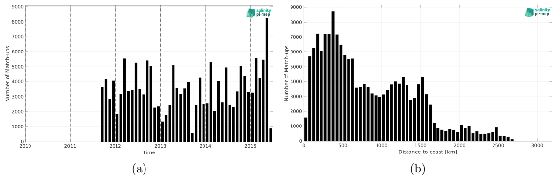
Figure 1: Number of match-ups between TSG (LEGOS-DM) and Aquarius SSS L3 CAP v5 - 7-Day running (JPL) SSS as a function of time (a) and as function of the distance to coast (b) over the Equatorial Ocean 10N-10S Pi-MEP region and for the full satellite product period.
