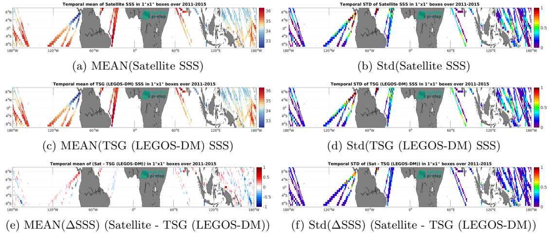
Figure 6: Temporal mean (left) and Std (right) of SSS from Aquarius SSS L3 CAP v5 - 7-Day running (JPL) (top), TSG (LEGOS-DM) (middle), and of \Delta SSS (Satellite - TSG (LEGOS-DM)). Only match-up pairs are used to generate these maps.
