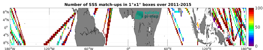
Figure 4: Number of SSS match-ups between TSG (LEGOS-DM) SSS and the Aquarius SSS L3 CAP v5 - 7-Day running (JPL) SSS product for the Equatorial Ocean 10N-10S Pi-MEP region over 1^\circ \times 1^\circ boxes and for the full satellite product period.
