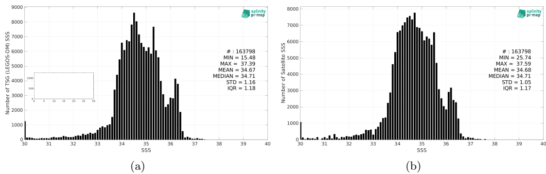
Figure 2: Histograms of SSS from TSG (LEGOS-DM) (a) and Aquarius SSS L3 CAP v5 - 7-Day running (JPL) (b) considering all match-up pairs per bins of 0.1 over the Equatorial Ocean 10N-10S Pi-MEP region and for the full satellite product period.
