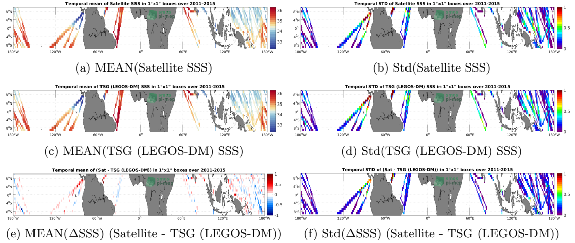
Figure 6: Temporal mean (left) and Std (right) of SSS from Aquarius SSS L3 CAP v5 - 7-Day running (JPL) (top), TSG (LEGOS-DM) in situ dataset (middle), and of \Delta SSS (Satellite - TSG (LEGOS-DM)). Only match-up pairs are used to generate these maps.
