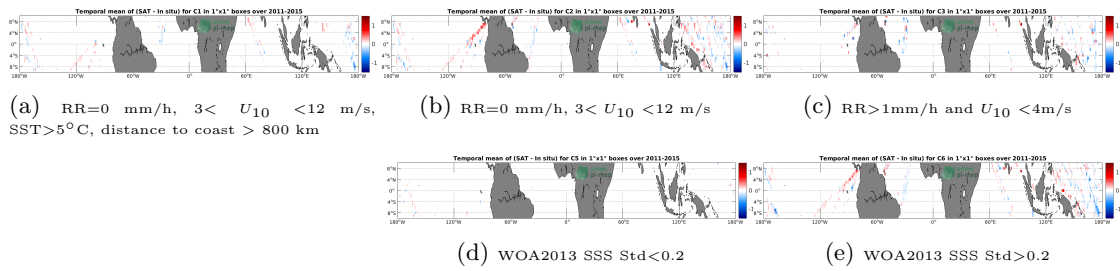
Figure 12: Temporal mean gridded over spatial boxes of size 1°x1° of \Delta SSS (Aquarius SSS L3 CAP v5 - 7-Day running (JPL) - TSG (LEGOS-DM)) for 5 different subdatasets corresponding to: RR=0 mm/h, 3 < U_{10} < 12 m/s, SST>5°C, distance to coast > 800 km (a), RR=0 mm/h, 3 < U_{10} < 12 m/s (b), RR>1mm/h and U_{10} < 4m/s (c), WOA2013 SSS Std<0.2 (d), WOA2013 SSS Std>0.2 (e).
