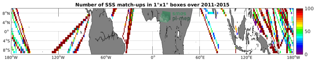
Figure 4: Number of SSS match-ups between TSG (LEGOS-DM) SSS and the Aquarius SSS L3 CAP v5 - 7-Day running (JPL) SSS product for the Equatorial Ocean 10N-10S Pi-MEP region over 1°x1° boxes and for the full satellite product period.
