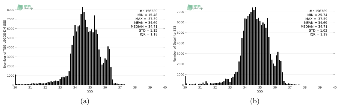
Figure 2: Histograms of SSS from TSG-LEGOS-DM (a) and Aquarius-L3-JPL-V5-7DAY-RUNNING (b) considering all match-up pairs per bins of 0.1 over the Equatorial Ocean 10N-10S Pi-MEP region and for the full satellite product period.
