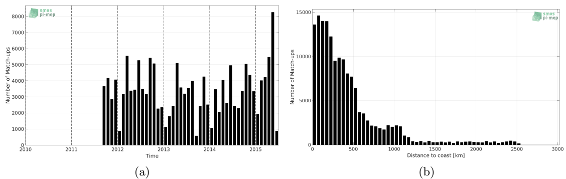
Figure 1: Number of match-ups between TSG-LEGOS-DM and Aquarius-L3-JPL-V5-7DAY-RUNNING SSS as a function of time (a) and as function of the distance to coast (b) over the Equatorial Ocean 10N-10S Pi-MEP region and for the full satellite product period.
