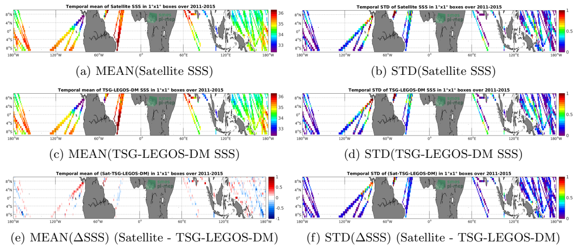
Figure 6: Temporal mean (left) and STD (right) of SSS from Aquarius-L3-JPL-V5-7DAY-RUNNING (top), TSG-LEGOS-DM (middle), and of \Delta SSS (Satellite - TSG-LEGOS-DM). Only match-up pairs are used to generate these maps.
