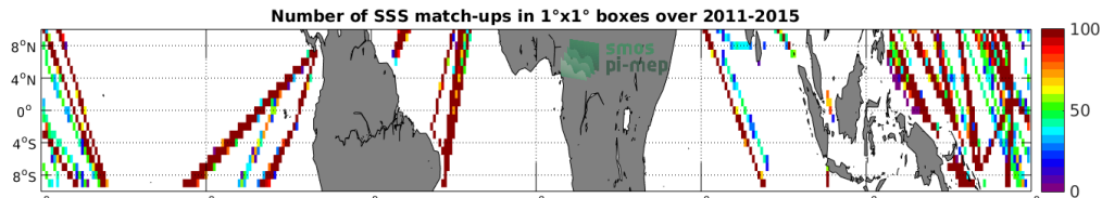
Figure 4: Number of SSS match-ups between TSG-LEGOS-DM SSS and the Aquarius-L3-JPL-V5-7DAY-RUNNING SSS product for the Equatorial Ocean 10N-10S Pi-MEP region over 1^\circ \times 1^\circ boxes and for the full satellite product period.
