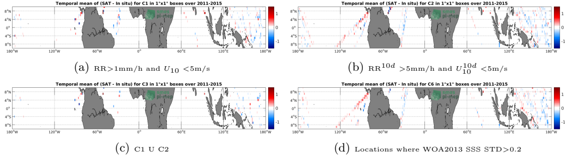
Figure 12: Temporal mean gridded over spatial boxes of size 1^\circ \times 1^\circ of \Delta SSS (Aquarius-L3-JPL-V5-7DAY-RUNNING - TSG-LEGOS-DM) for 4 different subdatasets corresponding to: RR > 1\text{mm/h} and U_{10} < 5\text{m/s} (a), RR^{10d} > 5\text{mm/h} and U_{10}^{10d} < 5\text{m/s} (b), C1 U C2 (c), Locations where WOA2013 SSS STD > 0.2 (d).
