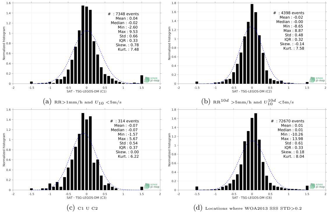
Figure 13: Normalized histogram of \Delta SSS (Aquarius-L3-JPL-V5-7DAY-RUNNING - TSG-LEGOS-DM) for 6 different subdatasets corresponding to: RR > 1\text{mm/h} and U_{10} < 5\text{m/s} (a), RR^{10d} > 5\text{mm/h} and U_{10}^{10d} < 5\text{m/s} (b), C1 U C2 (c), Locations where WOA2013 SSS STD > 0.2 (d).
