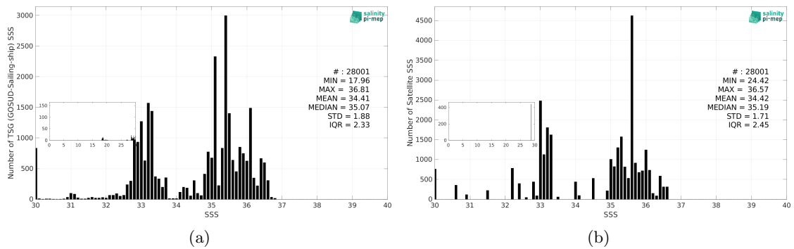
Figure 3: Histograms of SSS from TSG (GOSUD-Sailing-ship) (a) and Aquarius SSS L3 CAP v5 - 7-Day running (JPL) (b) considering all match-up pairs per bins of 0.1 over the Equatorial Ocean 10N-10S Pi-MEP region and for the full satellite product period.
