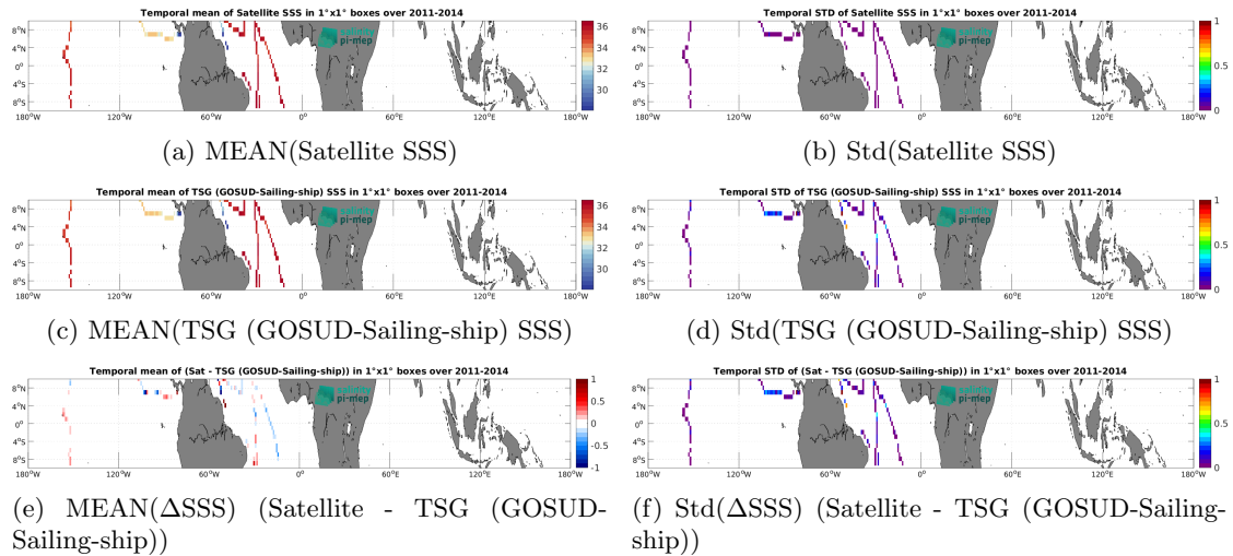
Figure 7: Temporal mean (left) and Std (right) of SSS from Aquarius SSS L3 CAP v5 - 7-Day running (JPL) (top), TSG (GOSUD-Sailing-ship) (middle), and of \Delta SSS (Satellite - TSG (GOSUD-Sailing-ship)). Only match-up pairs are used to generate these maps.
