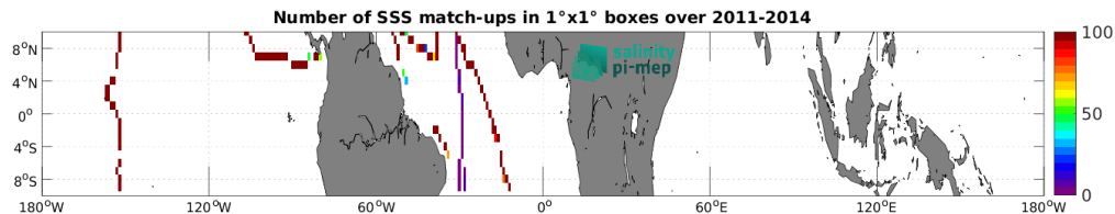
Figure 5: Number of SSS match-ups between TSG (GOSUD-Sailing-ship) SSS and the Aquarius SSS L3 CAP v5 - 7-Day running (JPL) SSS product for the Equatorial Ocean 10N-10S Pi-MEP region over 1^\circ \times 1^\circ boxes and for the full satellite product period.
