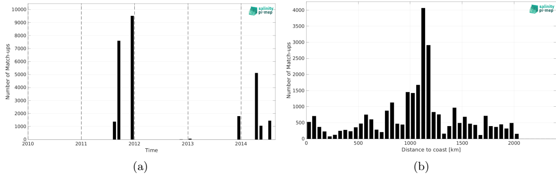
Figure 2: Number of match-ups between TSG (GOSUD-Sailing-ship) and Aquarius SSS L3 CAP v5 - 7-Day running (JPL) SSS as a function of time (a) and as function of the distance to coast (b) over the Equatorial Ocean 10N-10S Pi-MEP region and for the full satellite product period.
