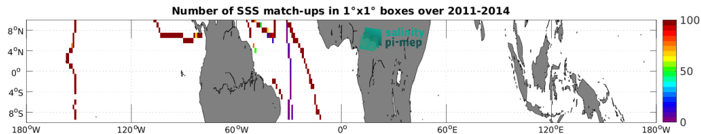
Figure 4: Number of SSS match-ups between TSG (GOSUD-Sailing-ship) SSS and the Aquarius SSS L3 CAP v5 - 7-Day running (JPL) SSS product for the Equatorial Ocean 10N-10S Pi-MEP region over 1^\circ \times 1^\circ boxes and for the full satellite product period.
