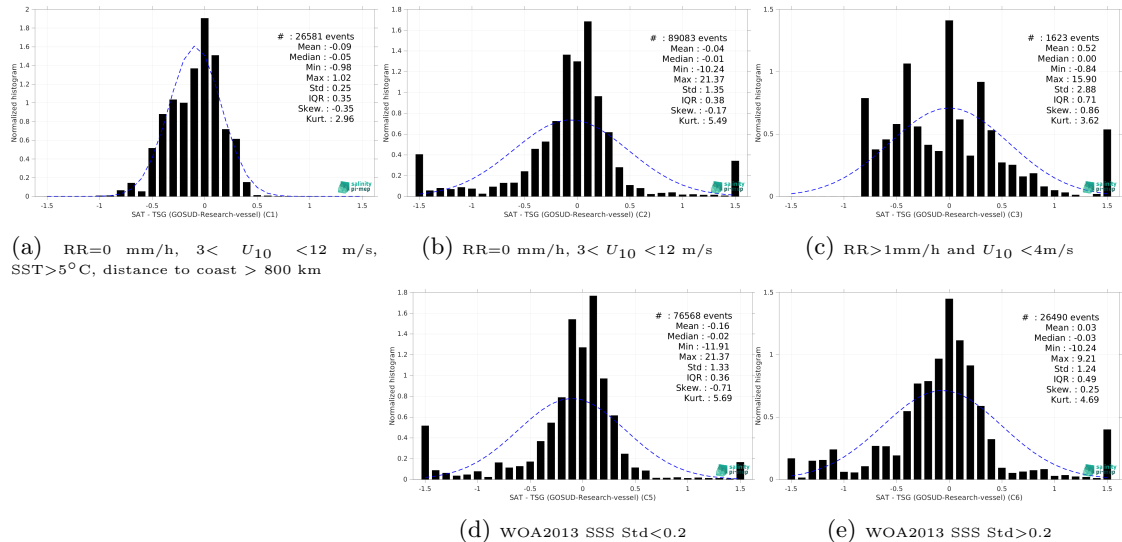
Figure 15: Normalized histogram of \Delta\text{SSS} (Aquarius SSS L3 CAP v5 - 7-Day running (JPL) - TSG (GOSUD-Research-vessel)) for 5 different subdatasets corresponding to: RR=0 mm/h, 3 < U_{10} < 12 m/s, SST>5°C, distance to coast > 800 km (a), RR=0 mm/h, 3 < U_{10} < 12 m/s (b), RR>1mm/h and U_{10} < 4 m/s (c), WOA2013 SSS Std<0.2 (d), WOA2013 SSS Std>0.2 (e).
