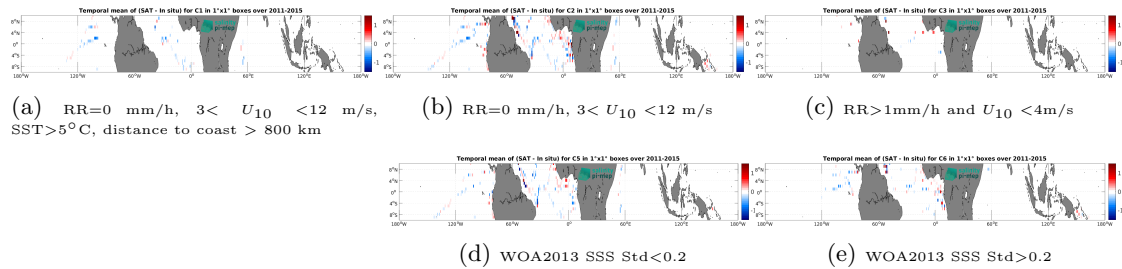
Figure 14: Temporal mean gridded over spatial boxes of size 1^\circ \times 1^\circ of \Delta\text{SSS} (Aquarius SSS L3 CAP v5 - 7-Day running (JPL) - TSG (GOSUD-Research-vessel)) for 5 different subdatasets corresponding to:RR=0 mm/h, 3 < U_{10} < 12 m/s, SST>5°C, distance to coast > 800 km (a), RR=0 mm/h, 3 < U_{10} < 12 m/s (b), RR>1mm/h and U_{10} < 4 m/s (c), WOA2013 SSS Std<0.2 (d), WOA2013 SSS Std>0.2 (e).
