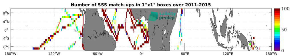
Figure 5: Number of SSS match-ups between TSG (GOSUD-Research-vessel) SSS and the Aquarius SSS L3 CAP v5 - 7-Day running (JPL) SSS product for the Equatorial Ocean 10N-10S Pi-MEP region over 1^\circ \times 1^\circ boxes and for the full satellite product period.
