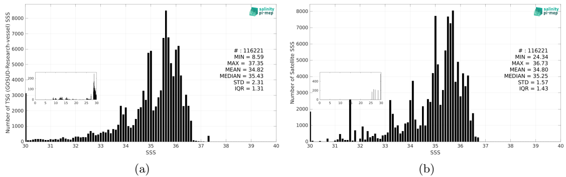
Figure 3: Histograms of SSS from TSG (GOSUD-Research-vessel) (a) and Aquarius SSS L3 CAP v5 - 7-Day running (JPL) (b) considering all match-up pairs per bins of 0.1 over the Equatorial Ocean 10N-10S Pi-MEP region and for the full satellite product period.
