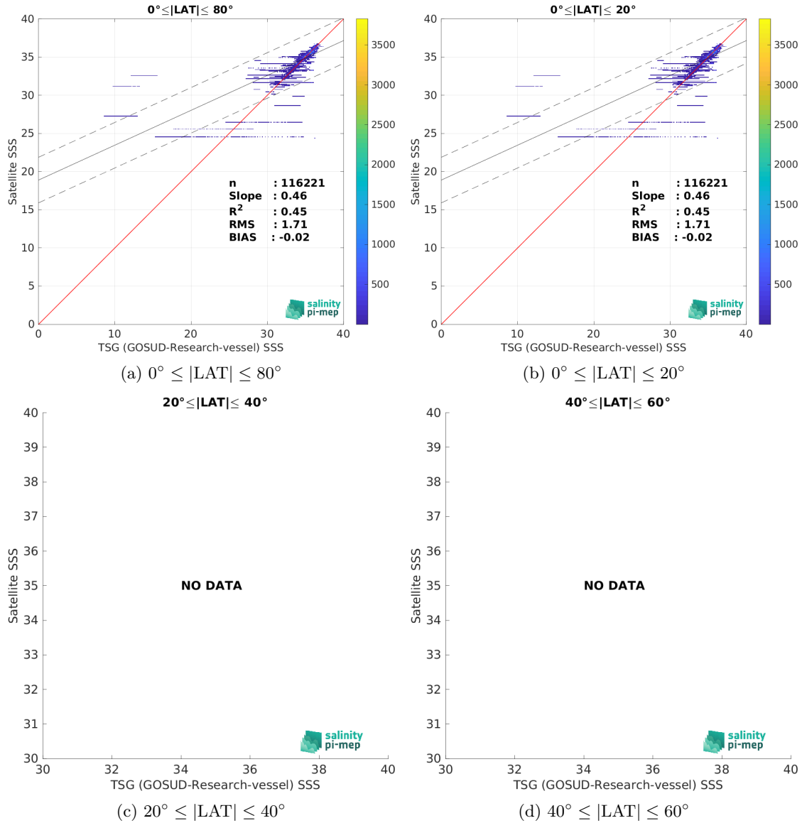
Figure 10: Contour maps of the concentration of Aquarius SSS L3 CAP v5 - 7-Day running (JPL) SSS (y-axis) versus TSG (GOSUD-Research-vessel) SSS (x-axis) at match-up pairs for different latitude bands. For each plot, the red line shows x=y . The black thin and dashed lines indicate a linear fit through the data cloud and the \pm 95\% confidence levels, respectively. The number match-up pairs n , the slope and R^2 coefficient of the linear fit, the root mean square (RMS) and the mean bias between satellite and in situ data are indicated for each latitude band in each plots.
