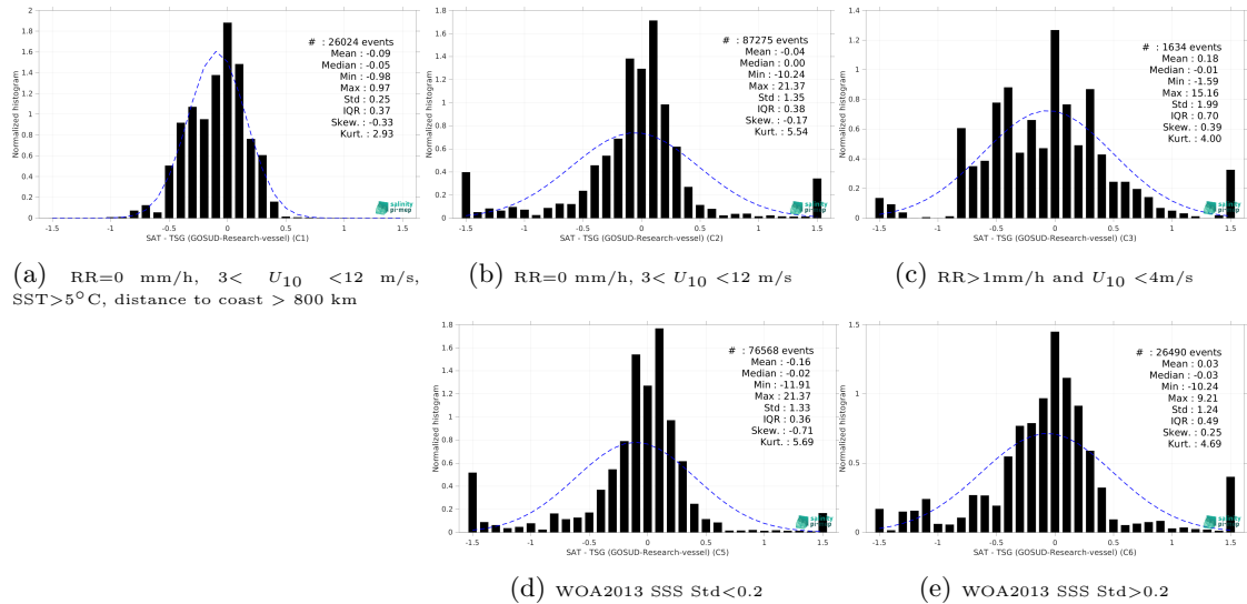
Figure 15: Normalized histogram of \Delta\text{SSS} (Aquarius SSS L3 CAP v5 - 7-Day running (JPL) - TSG (GOSUD-Research-vessel)) for 5 different subdatasets corresponding to: RR=0 mm/h, 3 < U_{10} < 12 m/s, SST>5°C, distance to coast > 800 km (a), RR=0 mm/h, 3 < U_{10} < 12 m/s (b), RR>1mm/h and U_{10} < 4 m/s (c), WOA2013 SSS Std<0.2 (d), WOA2013 SSS Std>0.2 (e).
