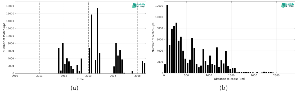
Figure 2: Number of match-ups between TSG (GOSUD-Research-vessel) and Aquarius SSS L3 CAP v5 - 7-Day running (JPL) SSS as a function of time (a) and as function of the distance to coast (b) over the Equatorial Ocean 10N-10S Pi-MEP region and for the full satellite product period.
