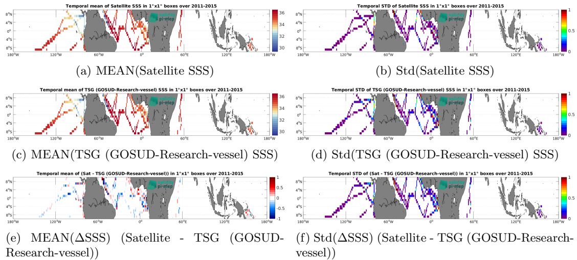
Figure 7: Temporal mean (left) and Std (right) of SSS from Aquarius SSS L3 CAP v5 - 7-Day running (JPL) (top), TSG (GOSUD-Research-vessel) (middle), and of \Delta SSS (Satellite - TSG (GOSUD-Research-vessel)). Only match-up pairs are used to generate these maps.
