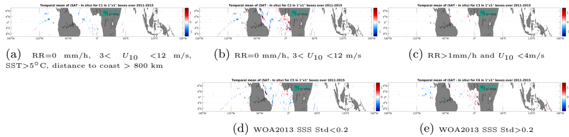
Figure 12: Temporal mean gridded over spatial boxes of size 1^\circ \times 1^\circ of \Delta\text{SSS} (Aquarius SSS L3 CAP v5 - 7-Day running (JPL) - TSG (GOSUD-Research-vessel)) for 5 different subdatasets corresponding to:RR=0 mm/h, 3 < U_{10} < 12 m/s, SST>5°C, distance to coast > 800 km (a), RR=0 mm/h, 3 < U_{10} < 12 m/s (b), RR>1mm/h and U_{10} < 4 m/s (c), WOA2013 SSS Std<0.2 (d), WOA2013 SSS Std>0.2 (e).
