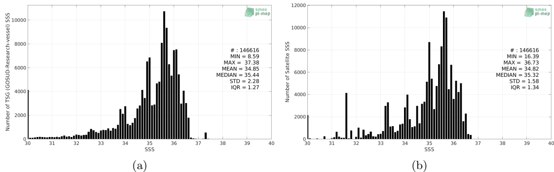
Figure 2: Histograms of SSS from TSG (GOSUD-Research-vessel) (a) and Aquarius SSS L3 CAP v5 - 7-Day running (JPL) (b) considering all match-up pairs per bins of 0.1 over the Equatorial Ocean 10N-10S Pi-MEP region and for the full satellite product period.
