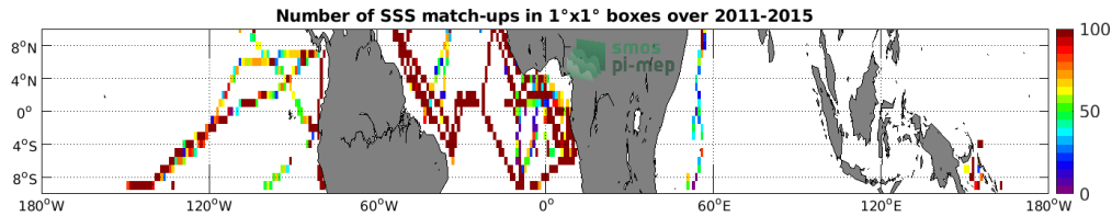
Figure 4: Number of SSS match-ups between TSG (GOSUD-Research-vessel) SSS and the Aquarius SSS L3 CAP v5 - 7-Day running (JPL) SSS product for the Equatorial Ocean 10N-10S Pi-MEP region over 1^\circ \times 1^\circ boxes and for the full satellite product period.
